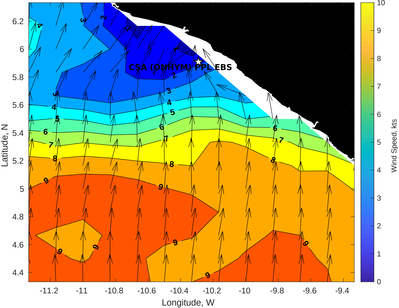
Winds (kts) for CSA (ONHYM) PPL EBS - Liberia at 30-Oct-2025 09:00:00
