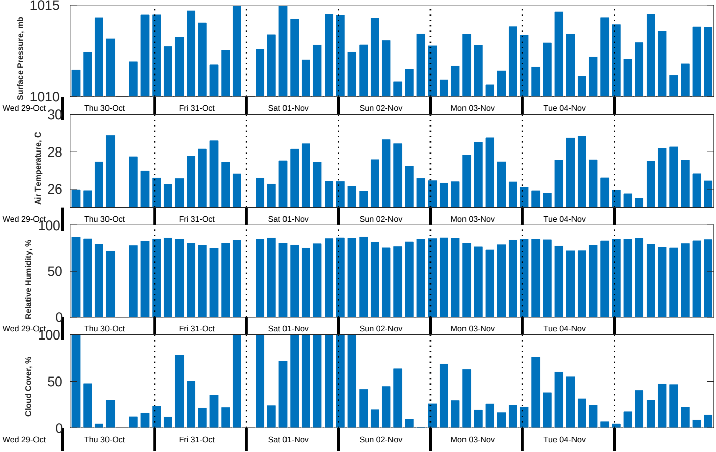
Met Forecast for CSA (ONHYM) PPL EBS - Liberia from 30-Oct-2025 00:00:00 to 06-Nov-2025 00:00:00
