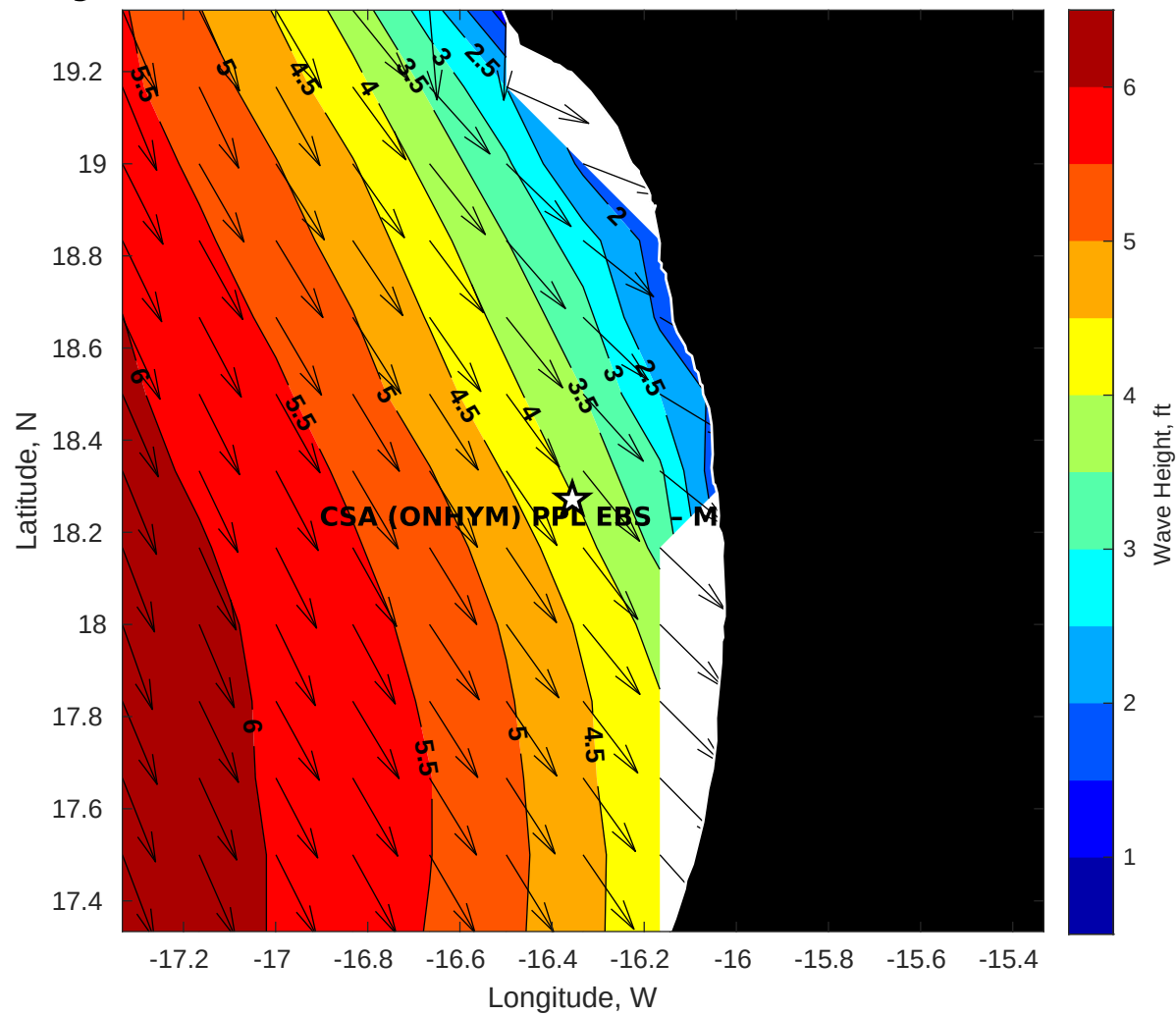
Wave Height (ft) for CSA (ONHYM) PPL EBS - Mauritania at 30-Oct-2025 09:00:00
