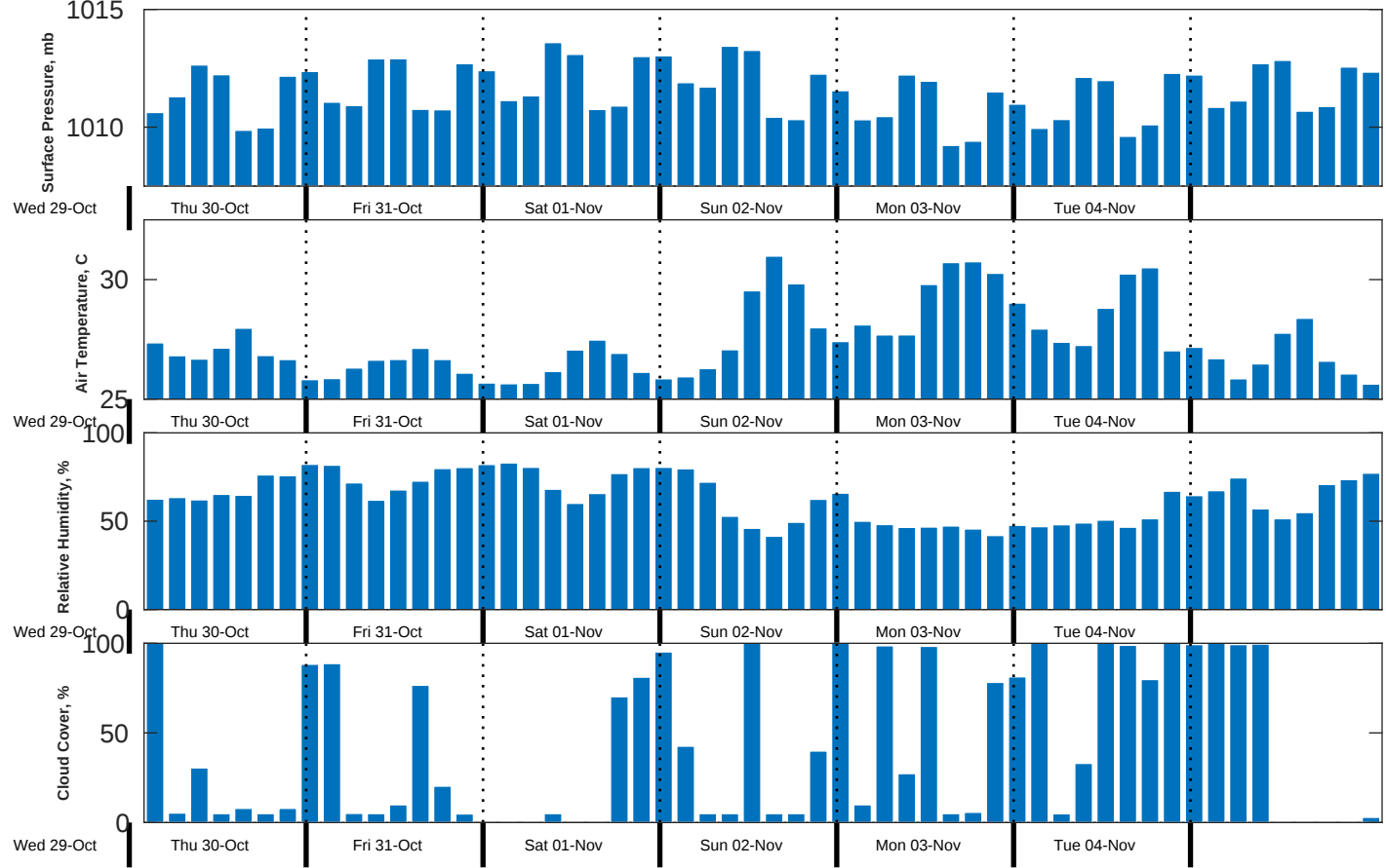
Met Forecast for CSA (ONHYM) PPL EBS - Mauritania from 30-Oct-2025 00:00:00 to 06-Nov-2025 00:00:00
