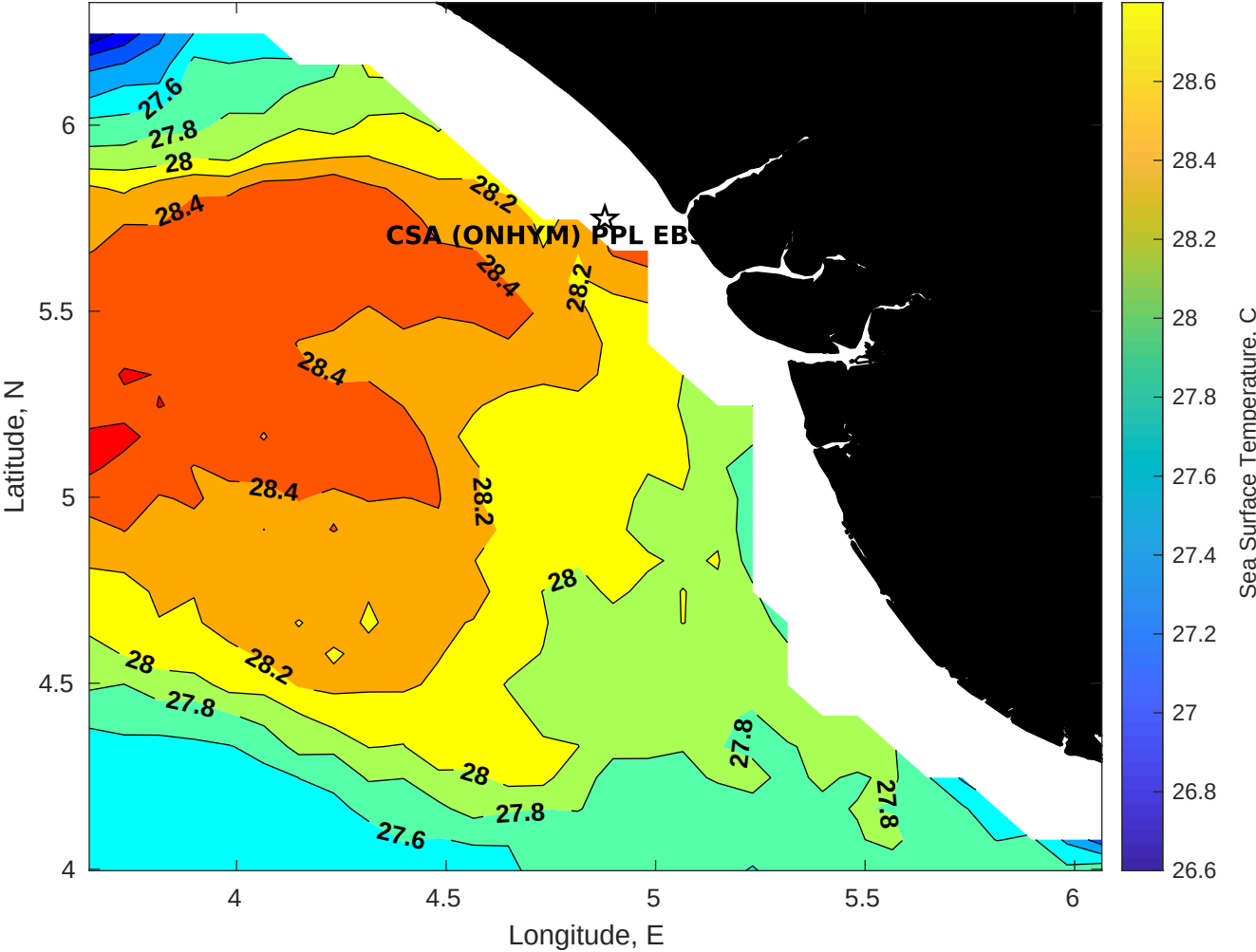
SST for CSA (ONHYM) PPL EBS - Nigeria at 29-Oct-2025 00:00:00
