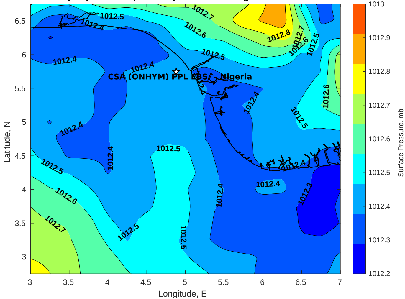
Surface Pressure (mb) for CSA (ONHYM) PPL EBS - Nigeria at 30-Oct-2025 00:00:00
