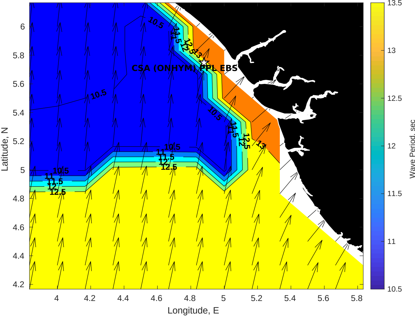
Wave Period (sec) for CSA (ONHYM) PPL EBS - Nigeria at 30-Oct-2025 09:00:00
