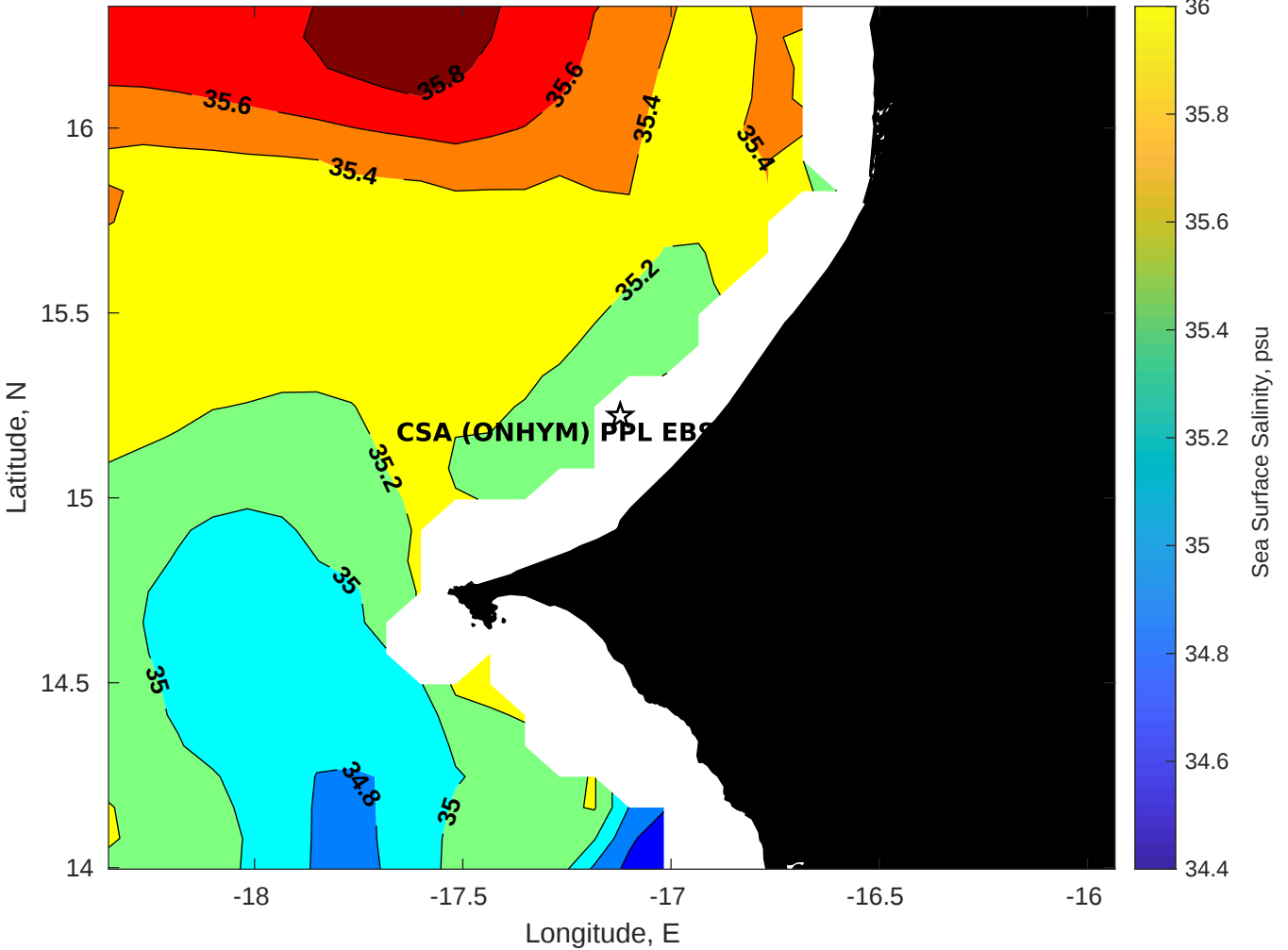
Surface Salinity for CSA (ONHYM) PPL EBS - Senegal at 29-Oct-2025 00:00:00
