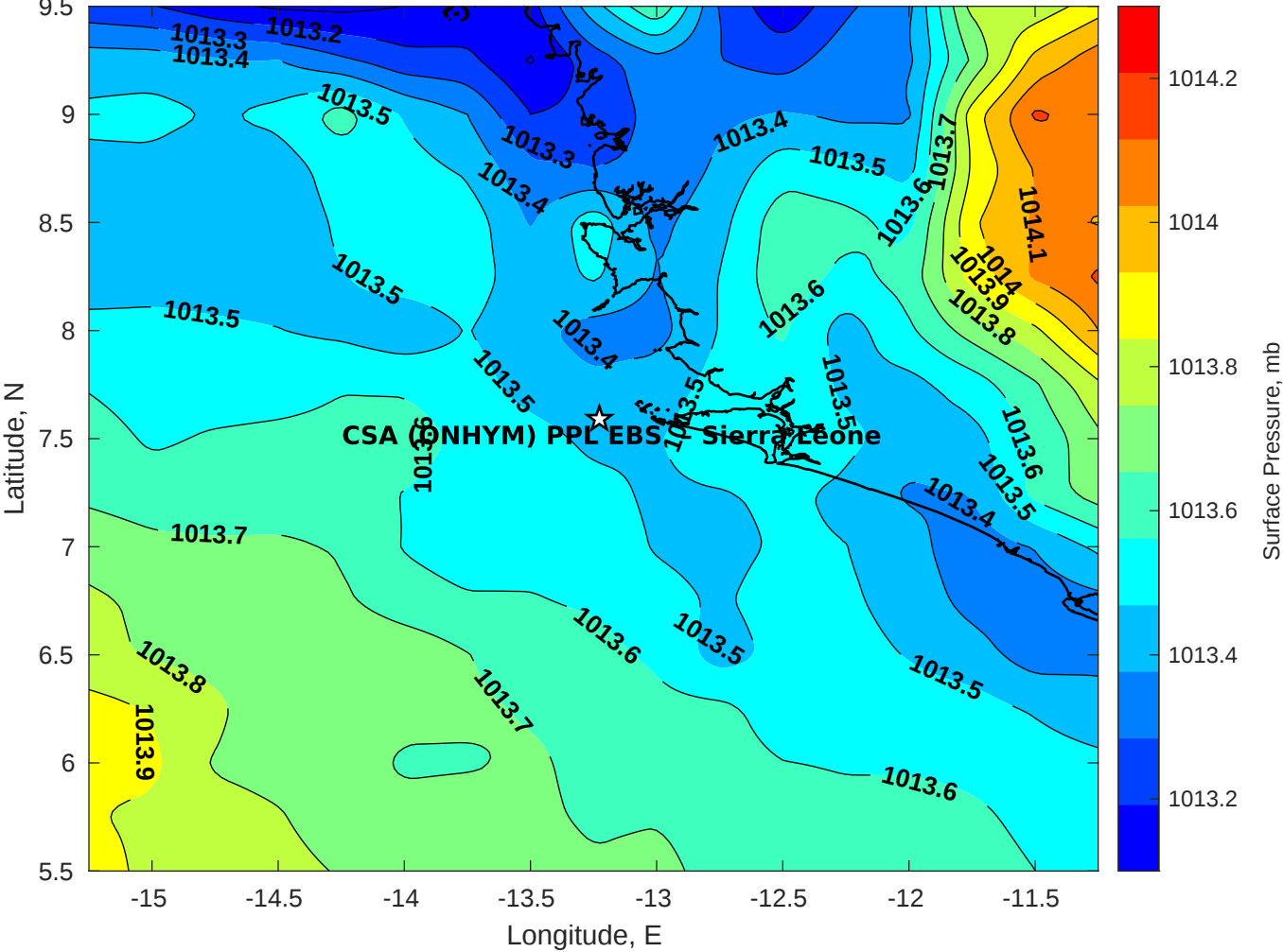
Surface Pressure (mb) for CSA (ONHYM) PPL EBS - Sierra Leone at 30-Oct-2025 00:00:00
