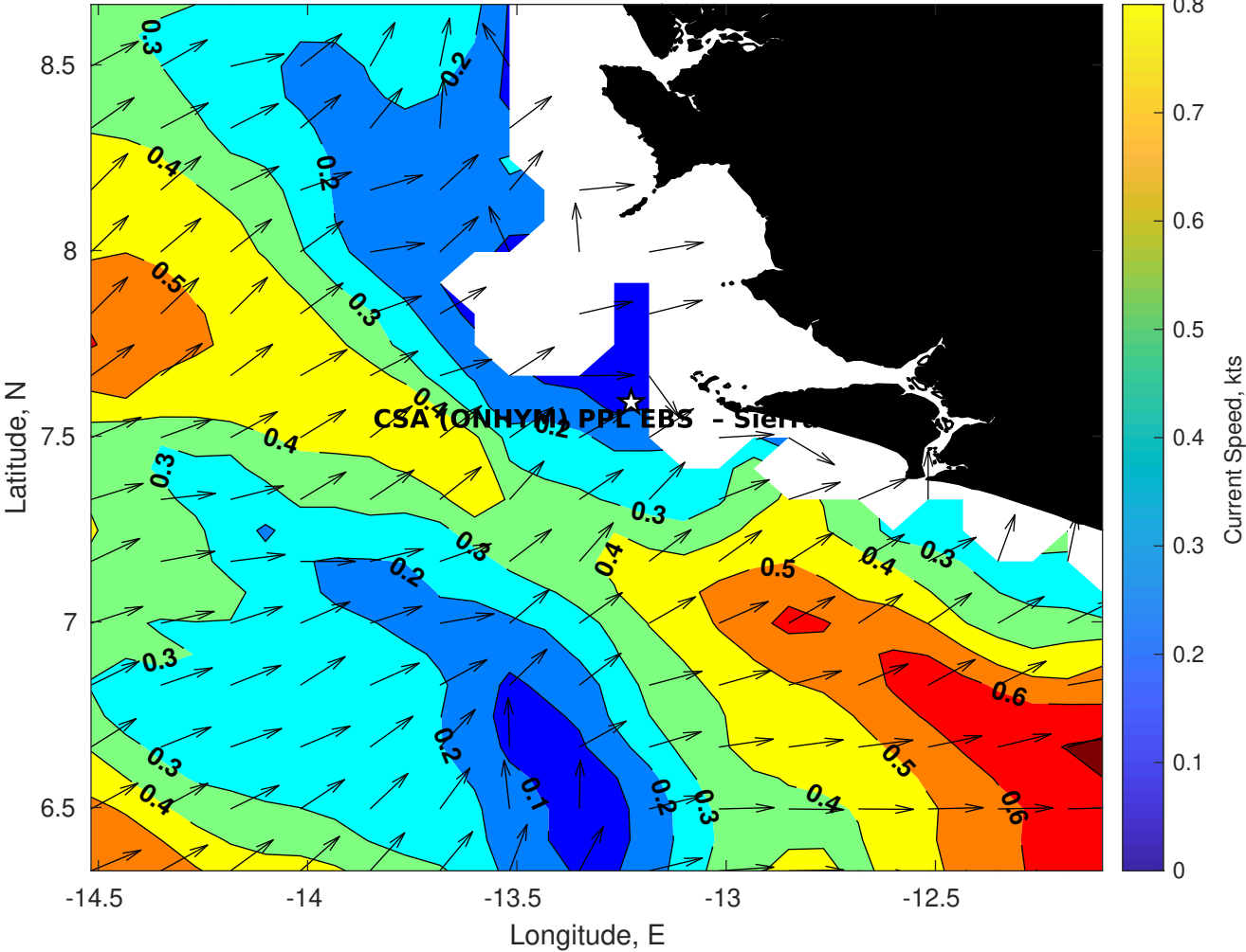
Surface Currents for CSA (ONHYM) PPL EBS - Sierra Leone at 29-Oct-2025 00:00:00
