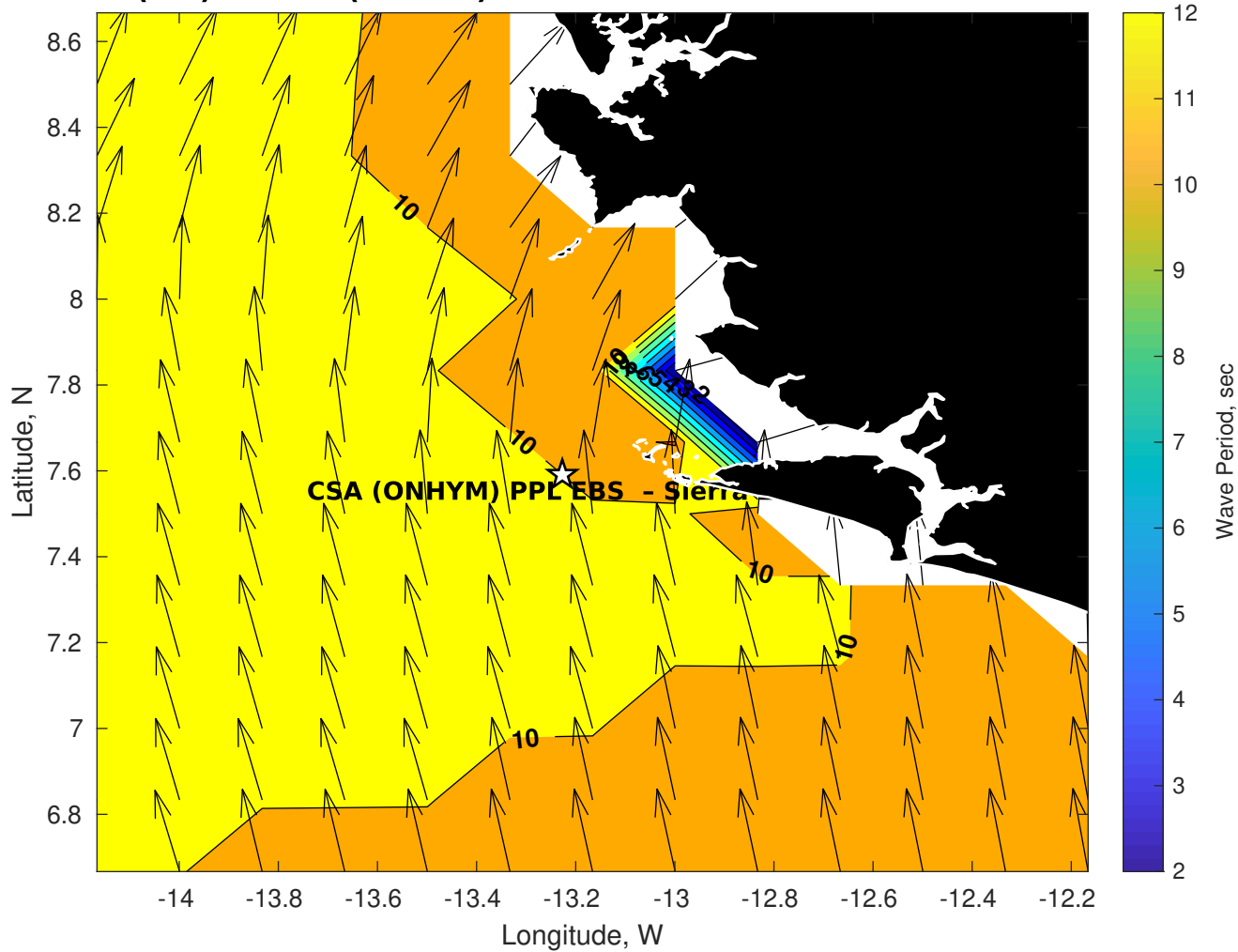
Wave Period (sec) for CSA (ONHYM) PPL EBS - Sierra Leone at 30-Oct-2025 09:00:00
