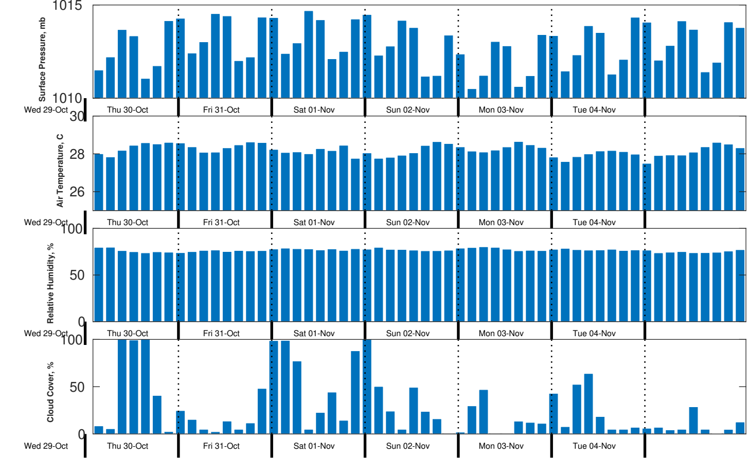
Met Forecast for CSA (ONHYM) PPL EBS - Sierra Leone from 30-Oct-2025 00:00:00 to 06-Nov-2025 00:00:00
