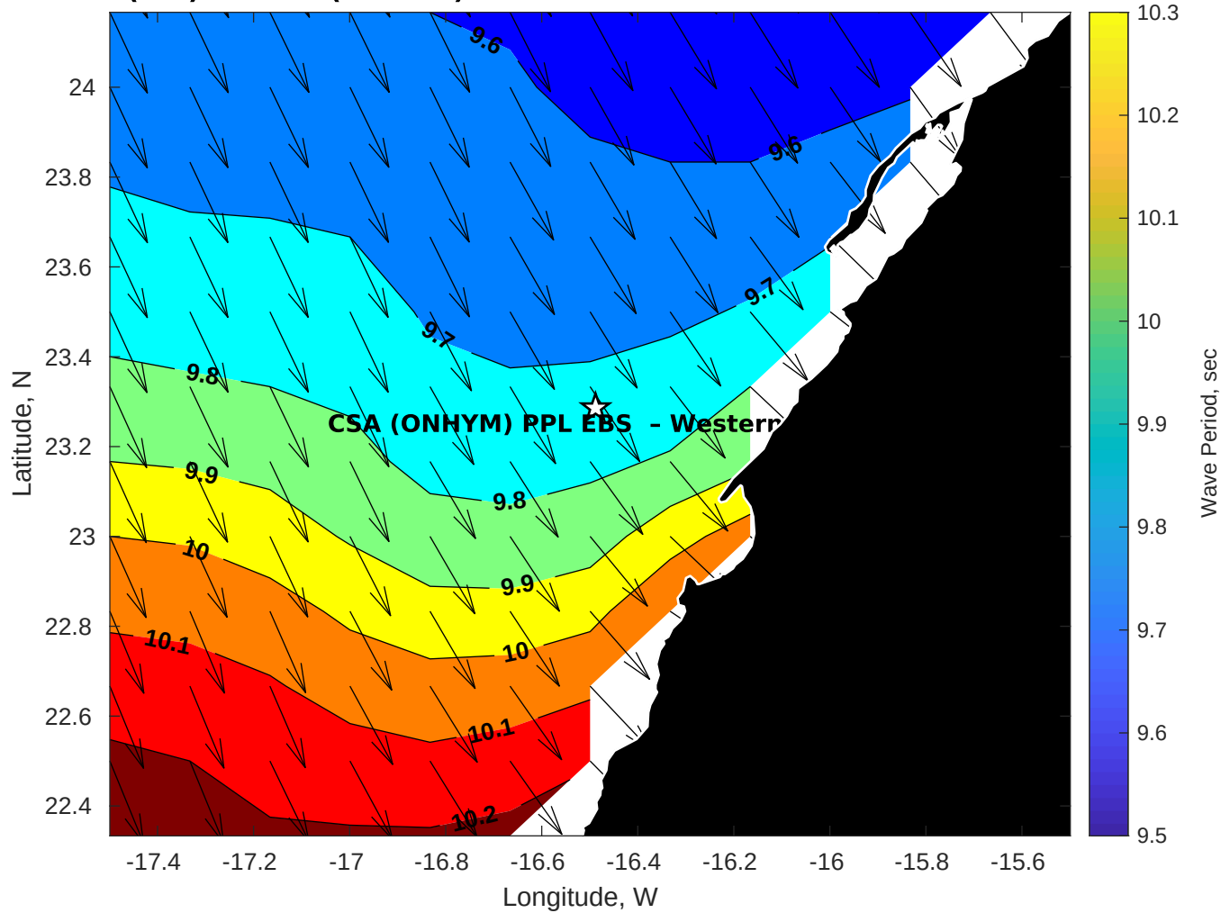
Wave Period (sec) for CSA (ONHYM) PPL EBS - Western Sahara at 30-Oct-2025 09:00:00
