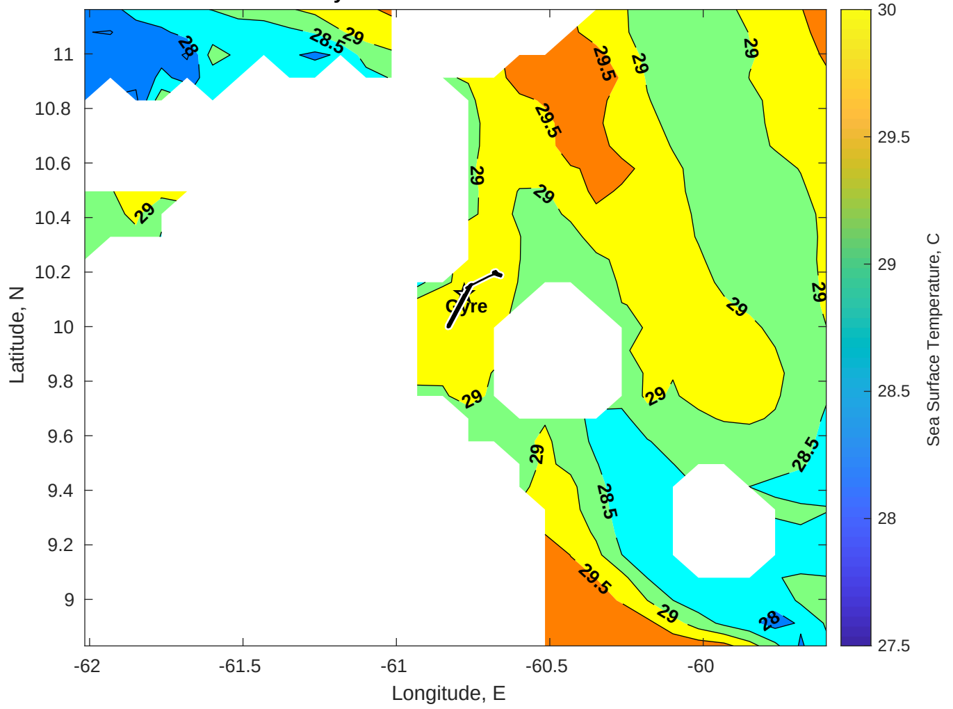
SST for Gyre at 29-Oct-2025 00:00:00
