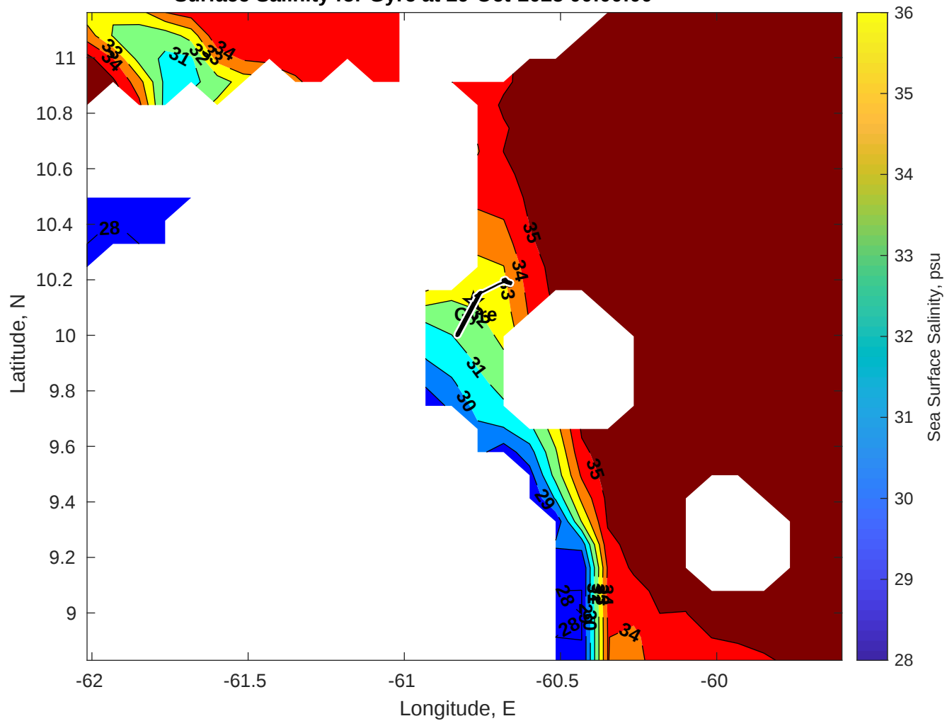
Surface Salinity for Gyre at 29-Oct-2025 00:00:00
