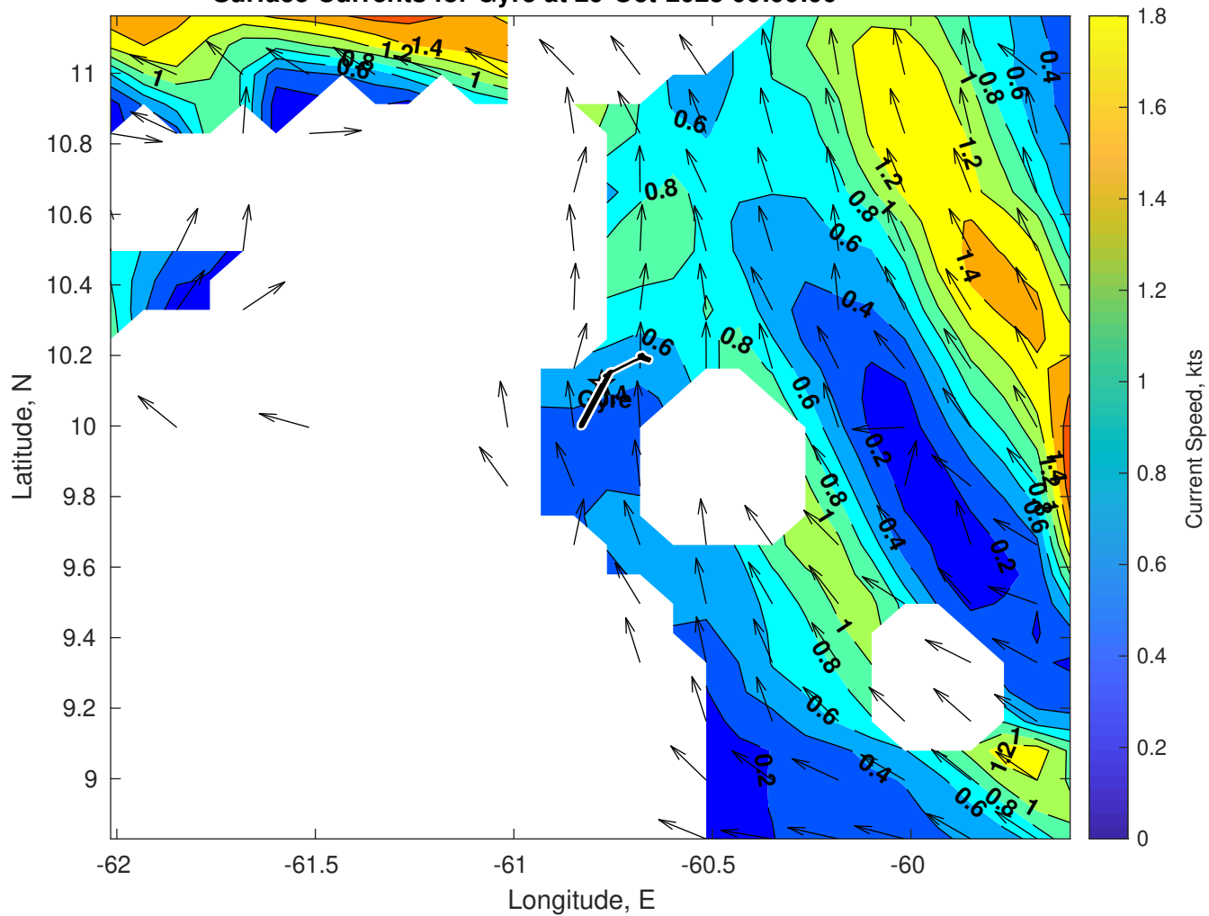
Surface Currents for Gyre at 29-Oct-2025 00:00:00
