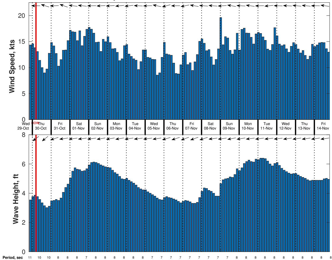
Wind & Wave Forecast for Gyre from 29-Oct-2025 20:00:00 to 14-Nov-2025 20:00:00
