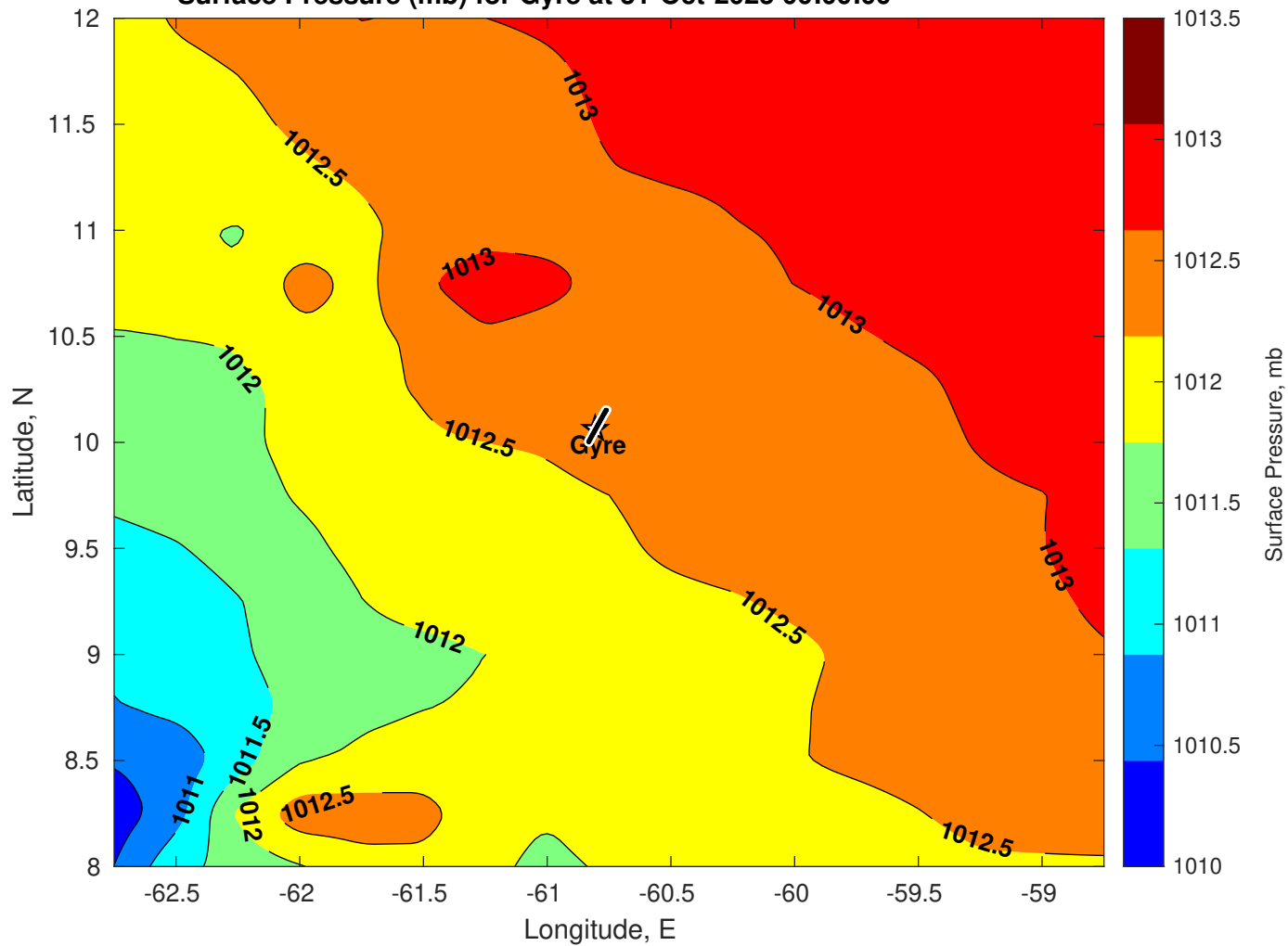
Surface Pressure (mb) for Gyre at 31-Oct-2025 00:00:00
