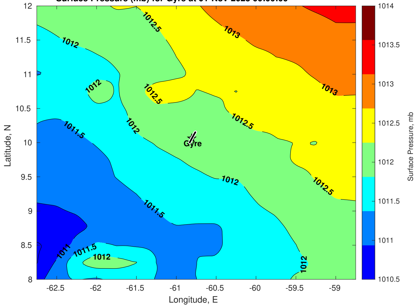
Surface Pressure (mb) for Gyre at 01-Nov-2025 00:00:00
