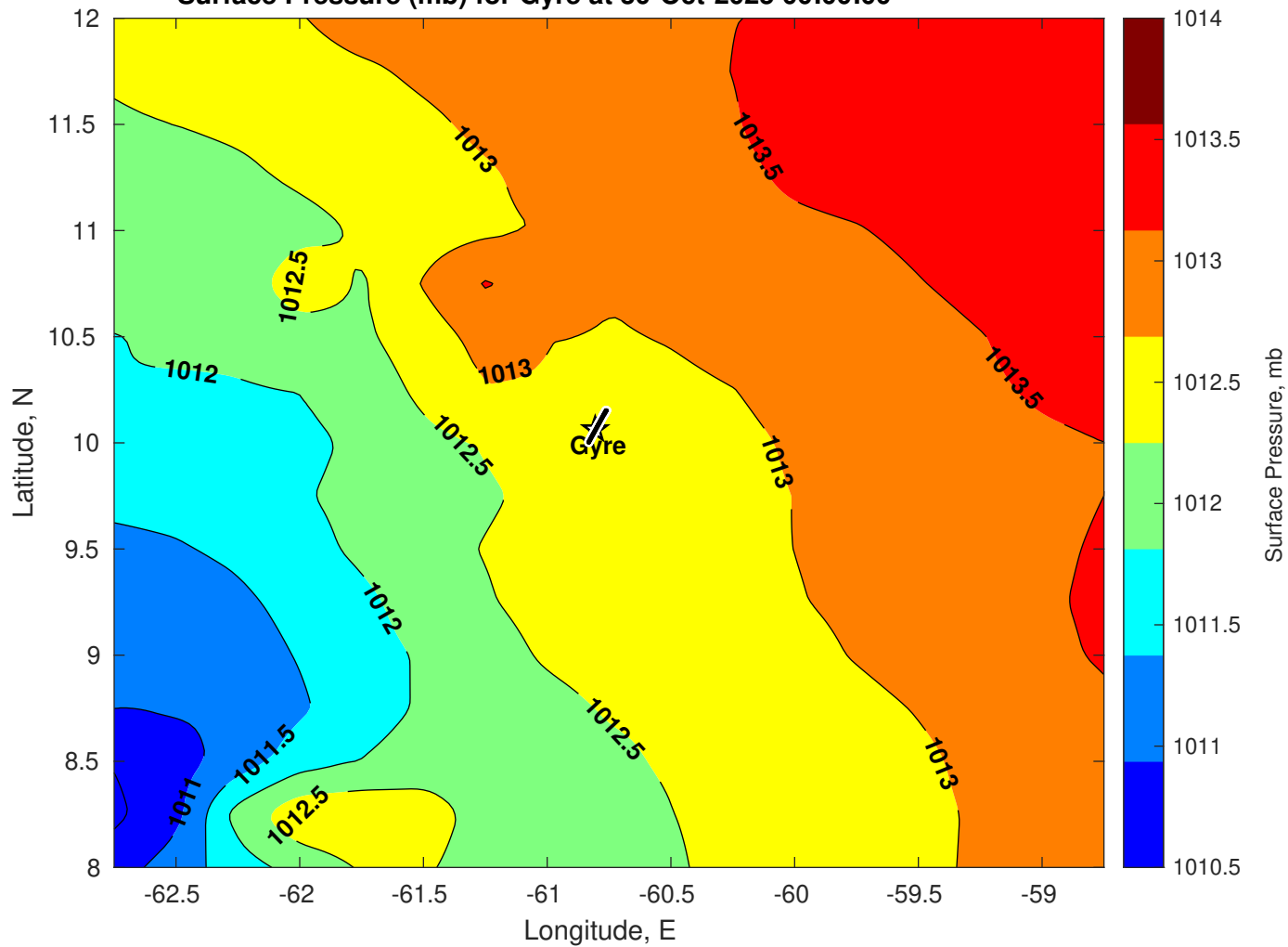
Surface Pressure (mb) for Gyre at 30-Oct-2025 00:00:00
