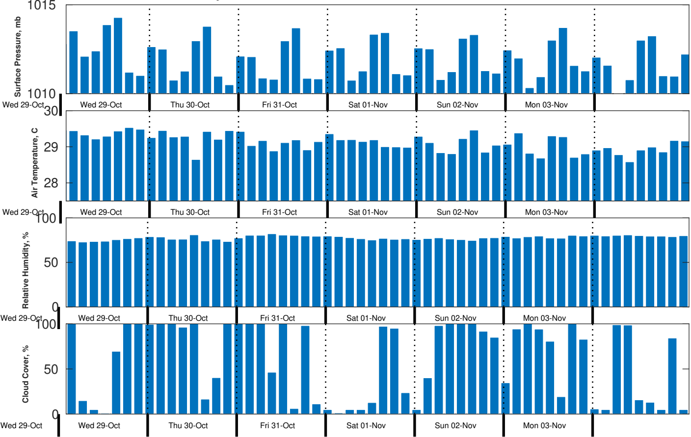
Met Forecast for Gyre from 29-Oct-2025 20:00:00 to 05-Nov-2025 20:00:00
