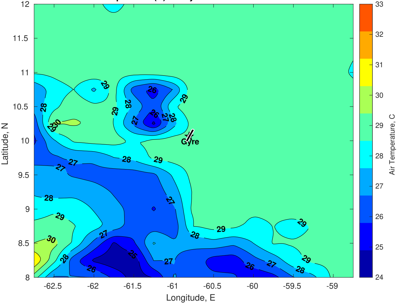
Air Temperature (C) for Gyre at 30-Oct-2025
