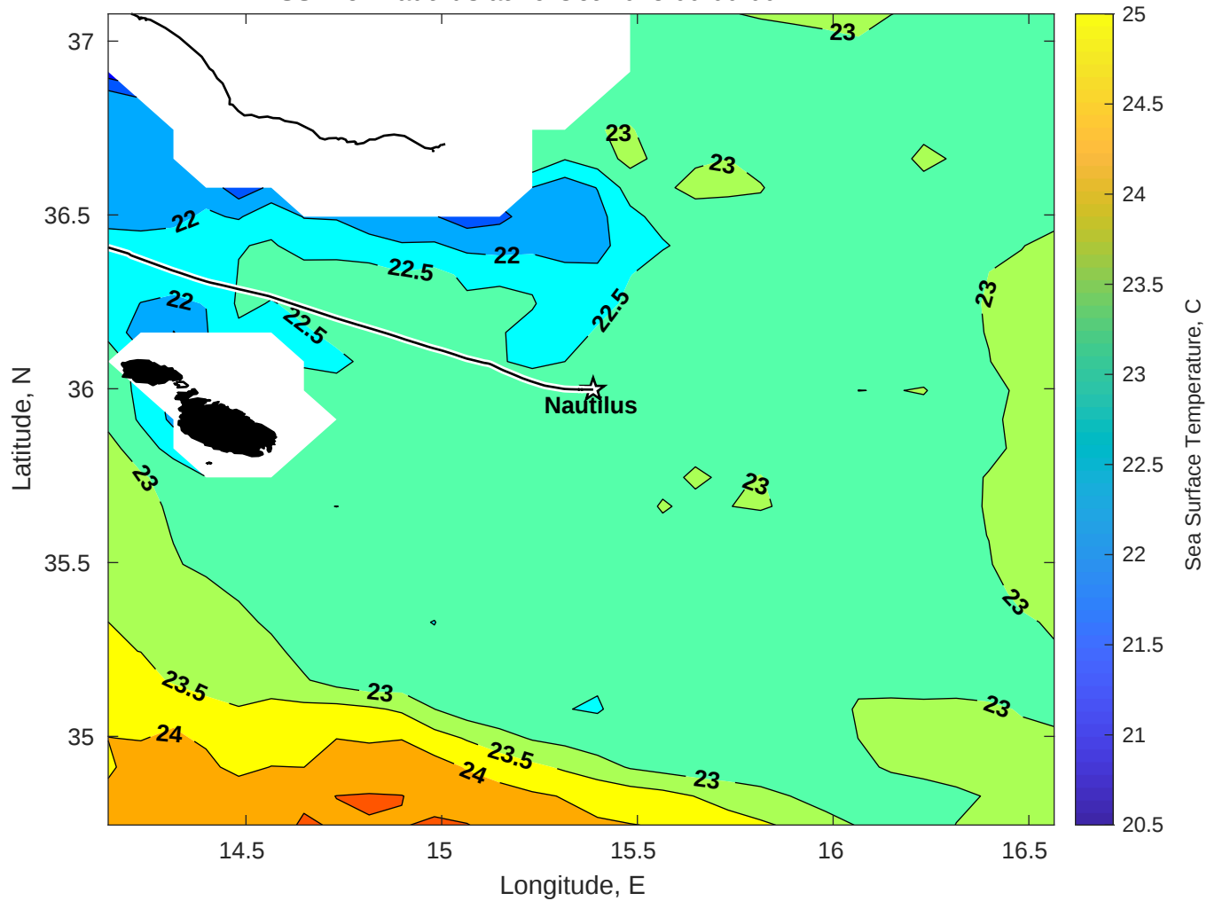
SST for Nautilus at 29-Oct-2025 00:00:00
