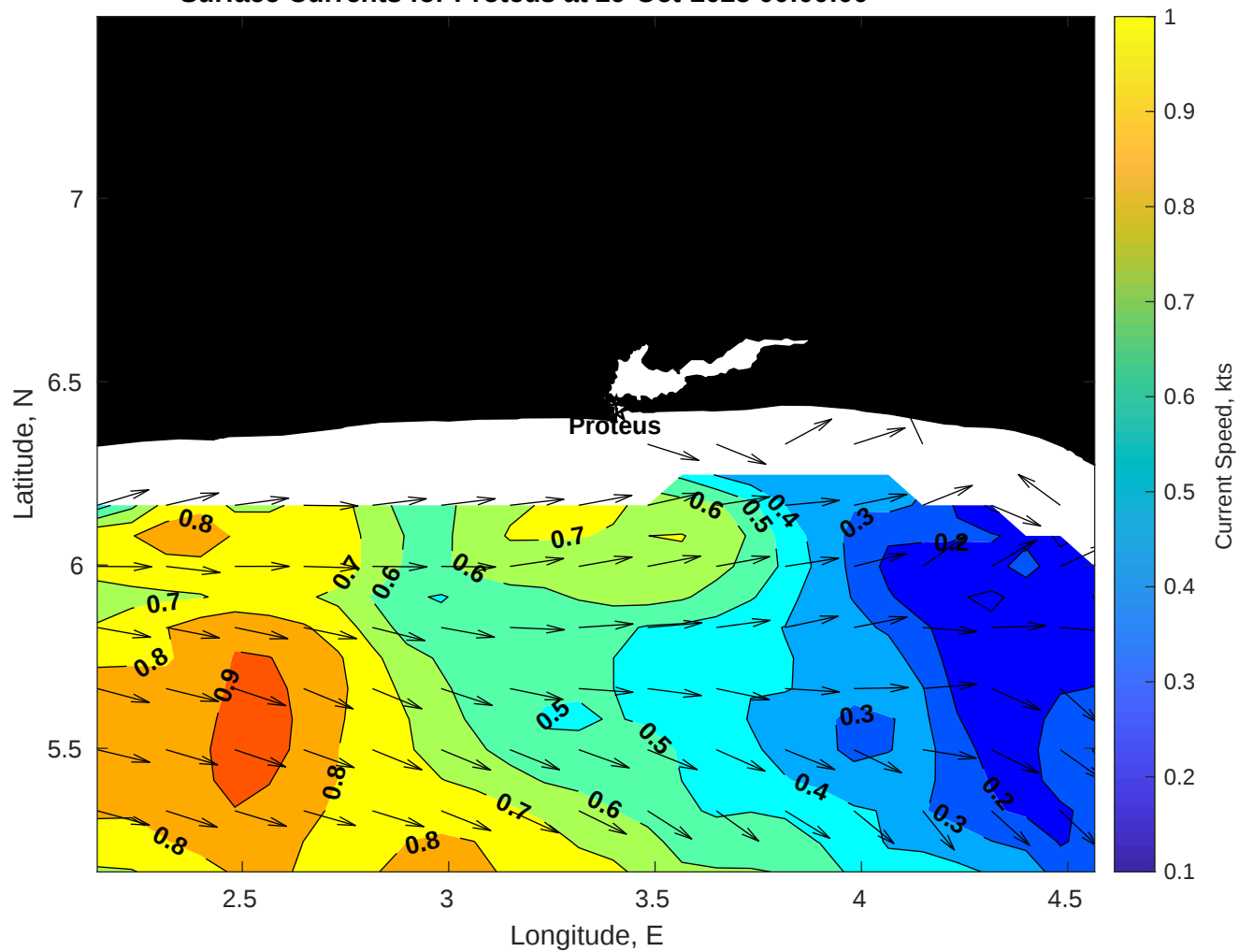
Surface Currents for Proteus at 29-Oct-2025 00:00:00
