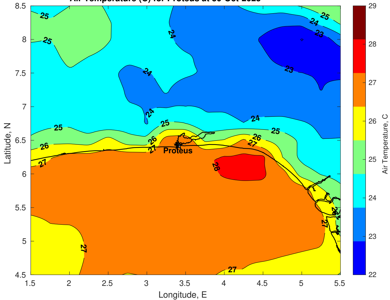
Air Temperature (C) for Proteus at 30-Oct-2025
