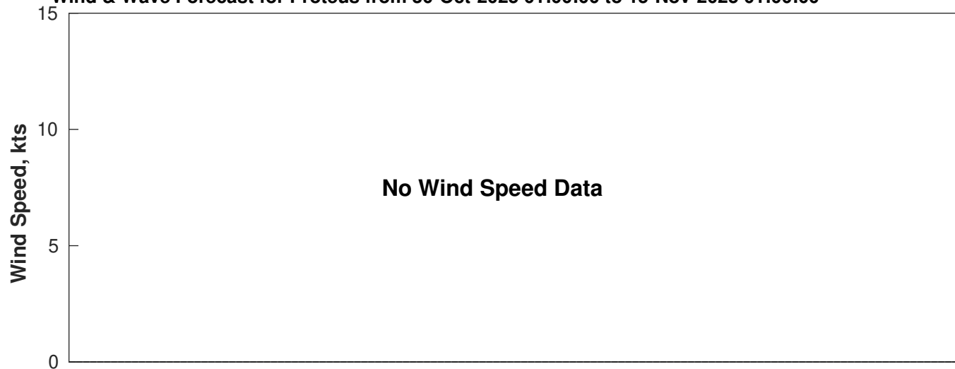
Wind & Wave Forecast for Proteus from 30-Oct-2025 01:00:00 to 15-Nov-2025 01:00:00
