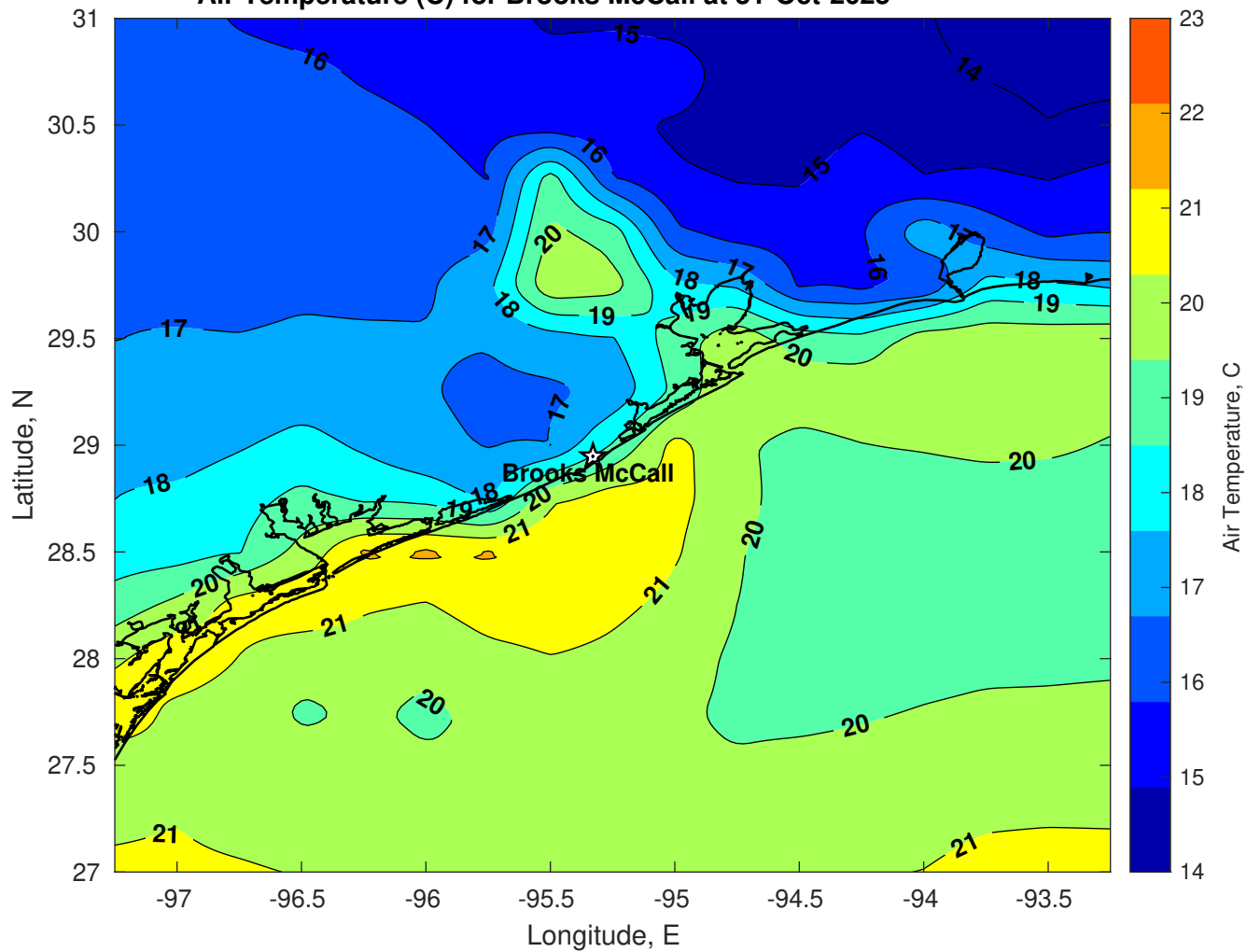
Air Temperature (C) for Brooks McCall at 31-Oct-2025
