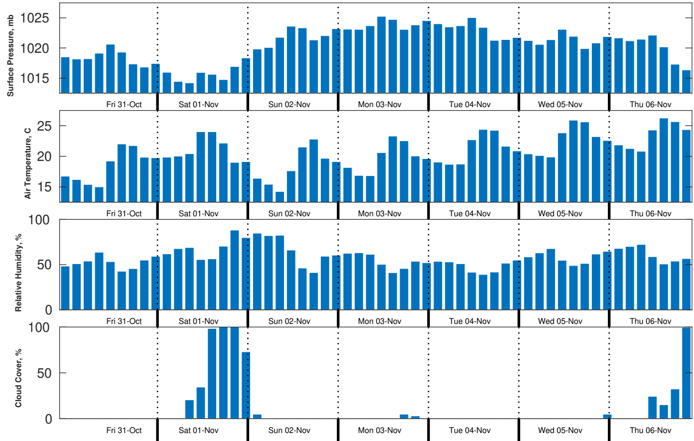
Met Forecast for Brooks McCall from 31-Oct-2025 00:00:00 to 07-Nov-2025 00:00:00
