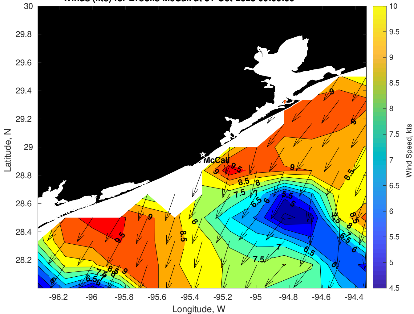
Winds (kts) for Brooks McCall at 31-Oct-2025 09:00:00
