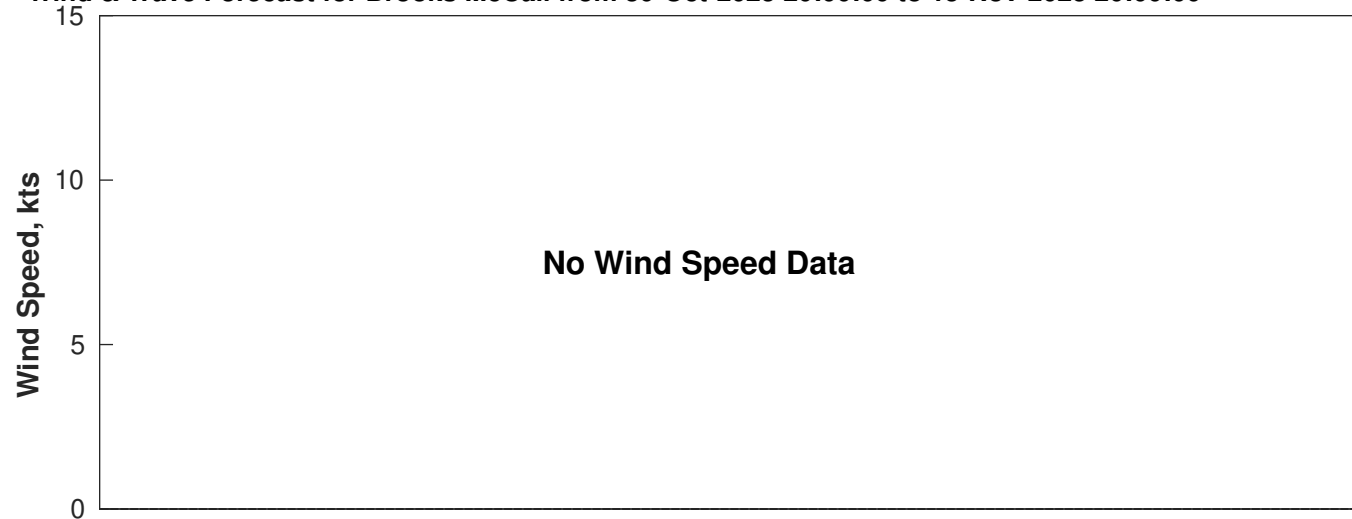
Wind & Wave Forecast for Brooks McCall from 30-Oct-2025 20:00:00 to 15-Nov-2025 20:00:00
