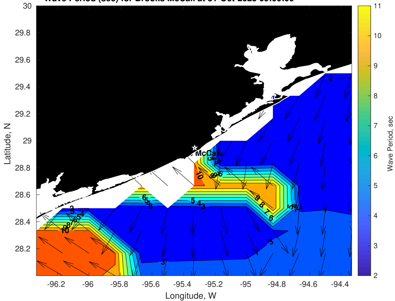
Wave Period (sec) for Brooks McCall at 31-Oct-2025 09:00:00
