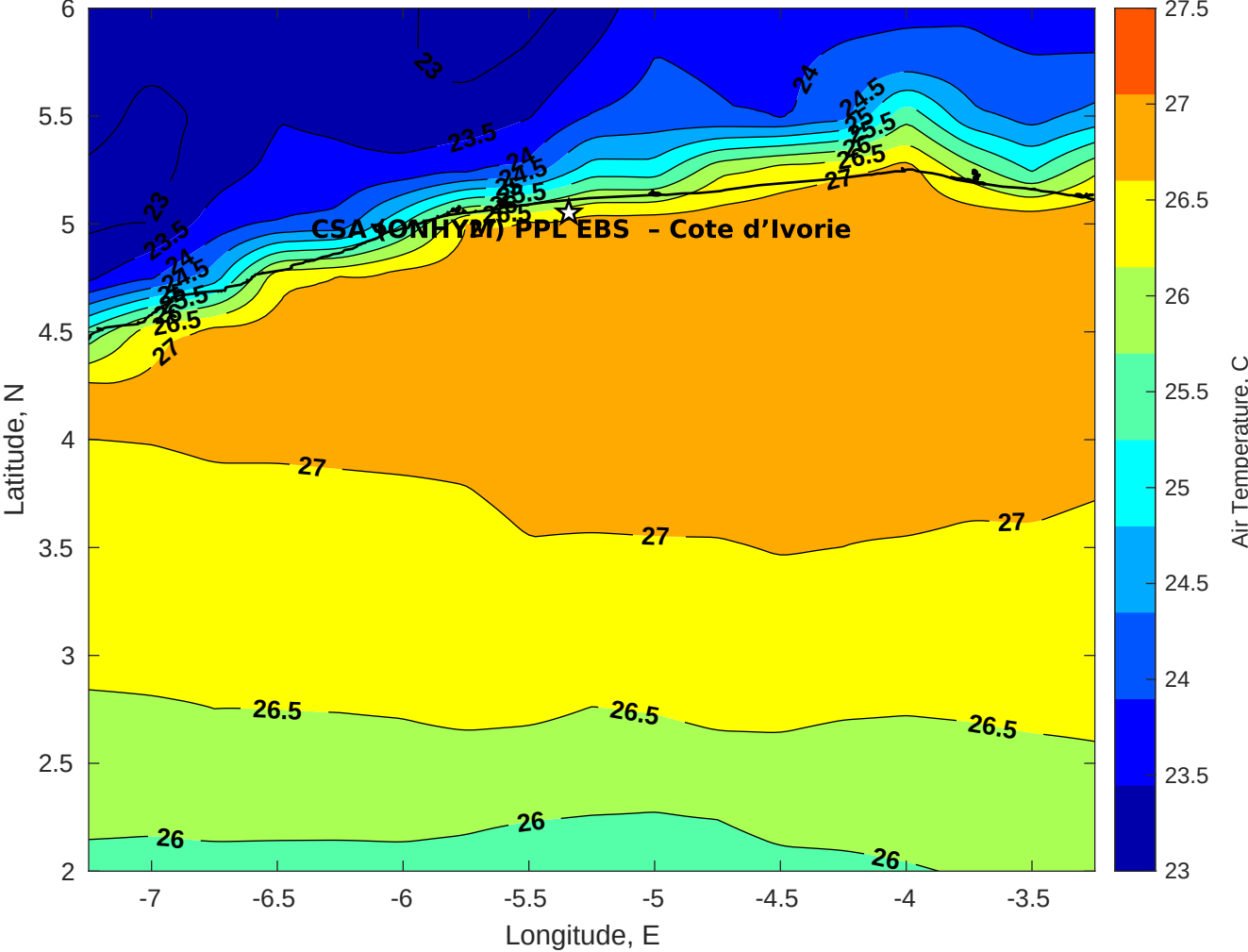
Air Temperature (C) for CSA (ONHYM) PPL EBS - Cote d'Ivoire at 31-Oct-2025
