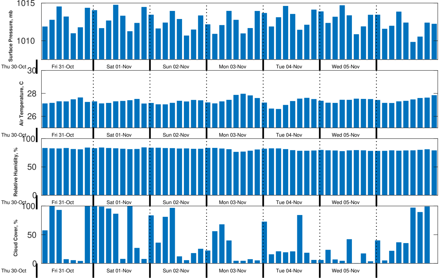
Met Forecast for CSA (ONHYM) PPL EBS - Cote d'Ivoire from 31-Oct-2025 00:00:00 to 07-Nov-2025 00:00:00
