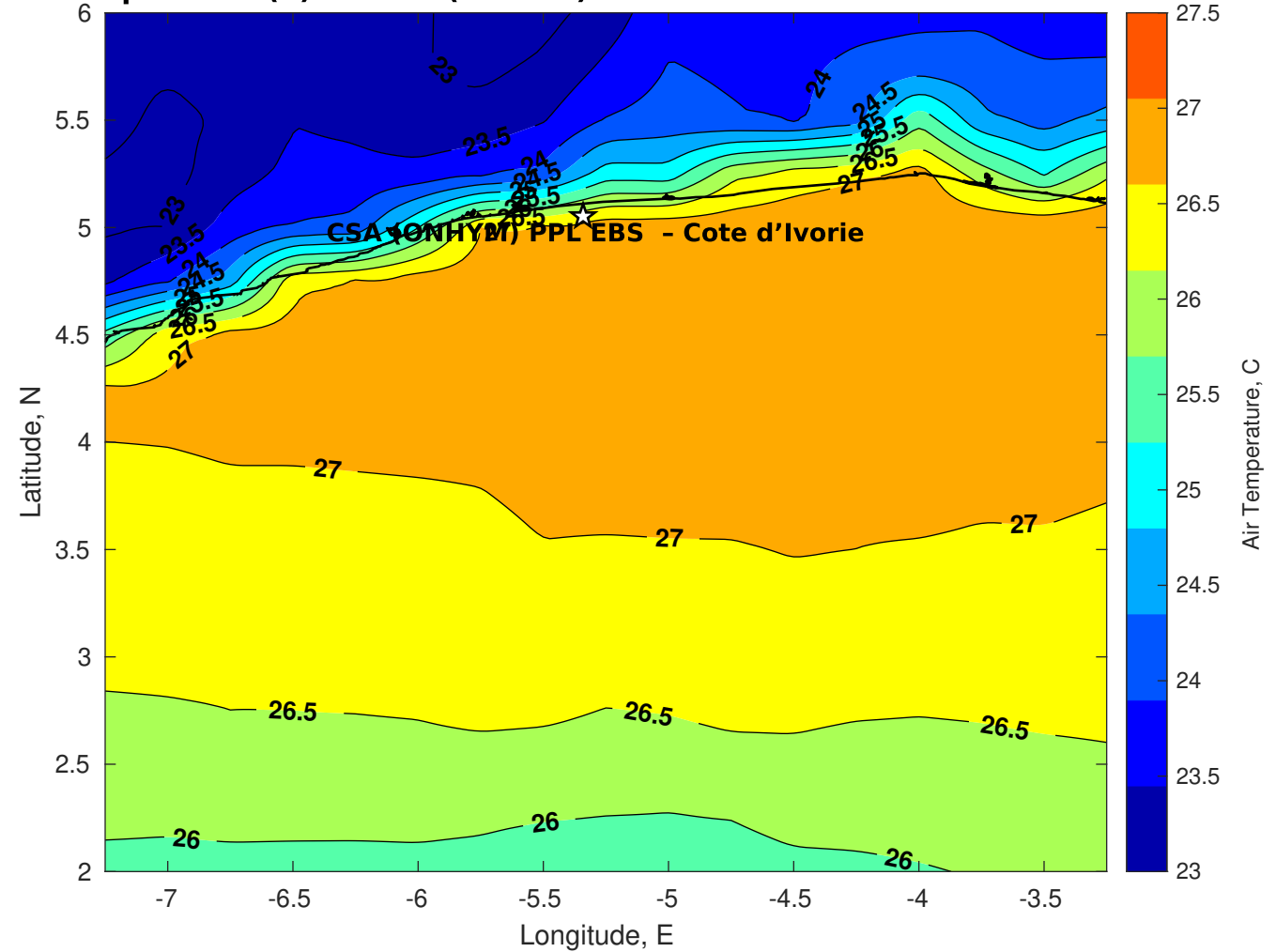
Air Temperature (C) for CSA (ONHYM) PPL EBS - Cote d'Ivoire at 31-Oct-2025
