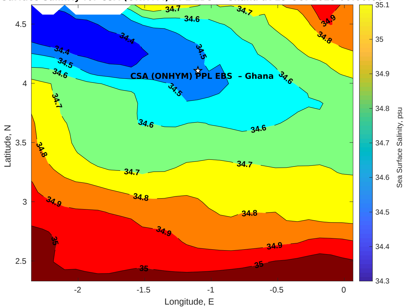
Surface Salinity for CSA (ONHYM) PPL EBS - Ghana at 29-Oct-2025 00:00:00
