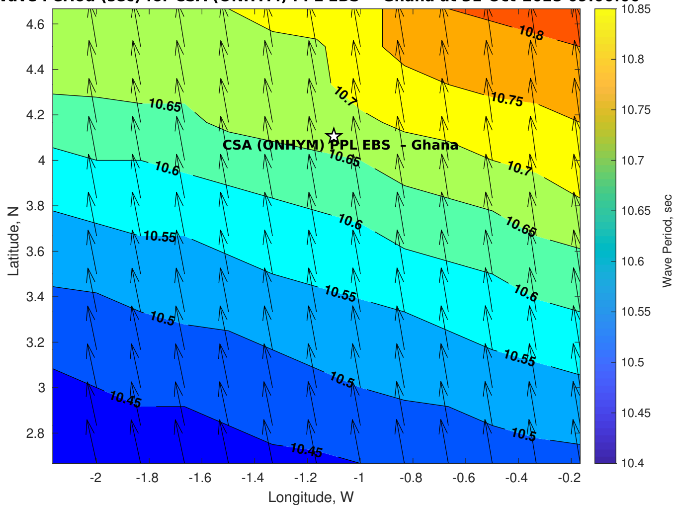
Wave Period (sec) for CSA (ONHYM) PPL EBS - Ghana at 31-Oct-2025 09:00:00
