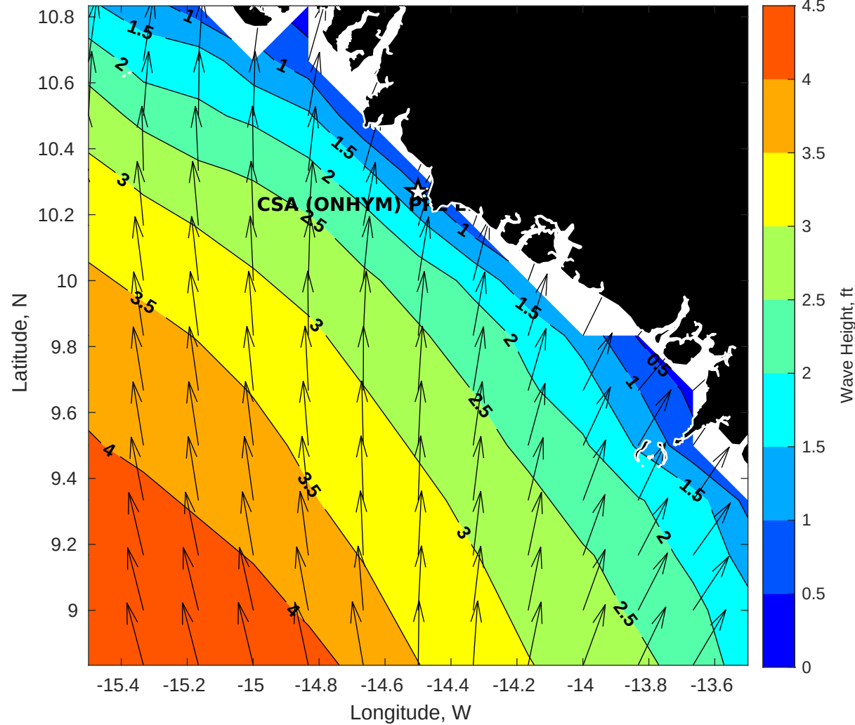
Wave Height (ft) for CSA (ONHYM) PPL EBS - Guinea at 31-Oct-2025 09:00:00
