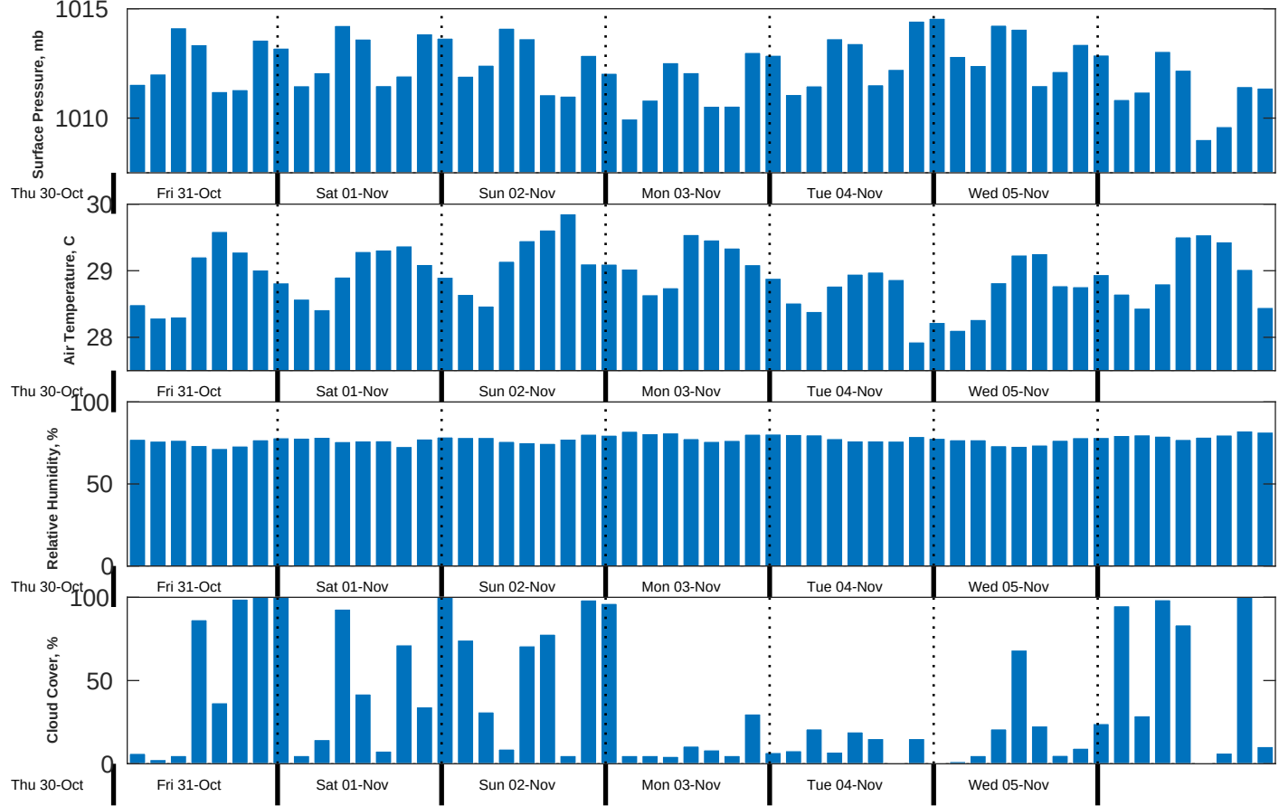
Met Forecast for CSA (ONHYM) PPL EBS - Guinea from 31-Oct-2025 00:00:00 to 07-Nov-2025 00:00:00
