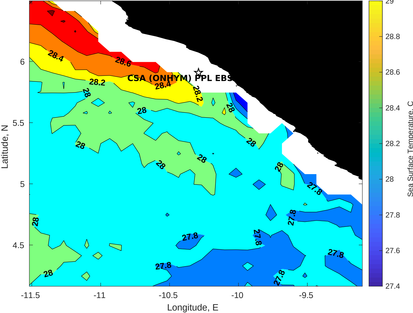
SST for CSA (ONHYM) PPL EBS - Liberia at 29-Oct-2025 00:00:00
