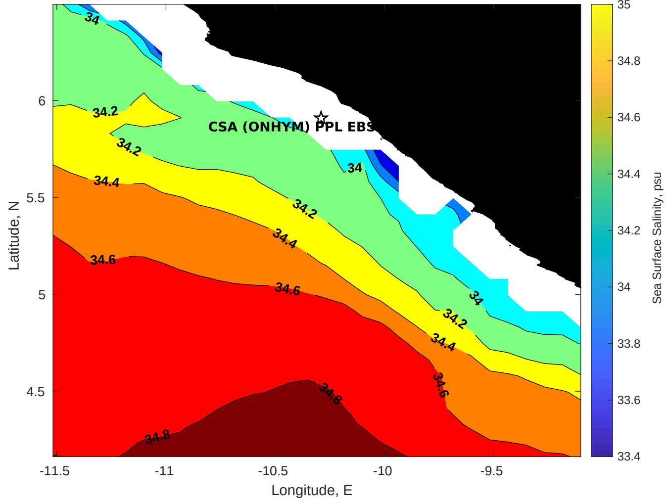
Surface Salinity for CSA (ONHYM) PPL EBS - Liberia at 29-Oct-2025 00:00:00
