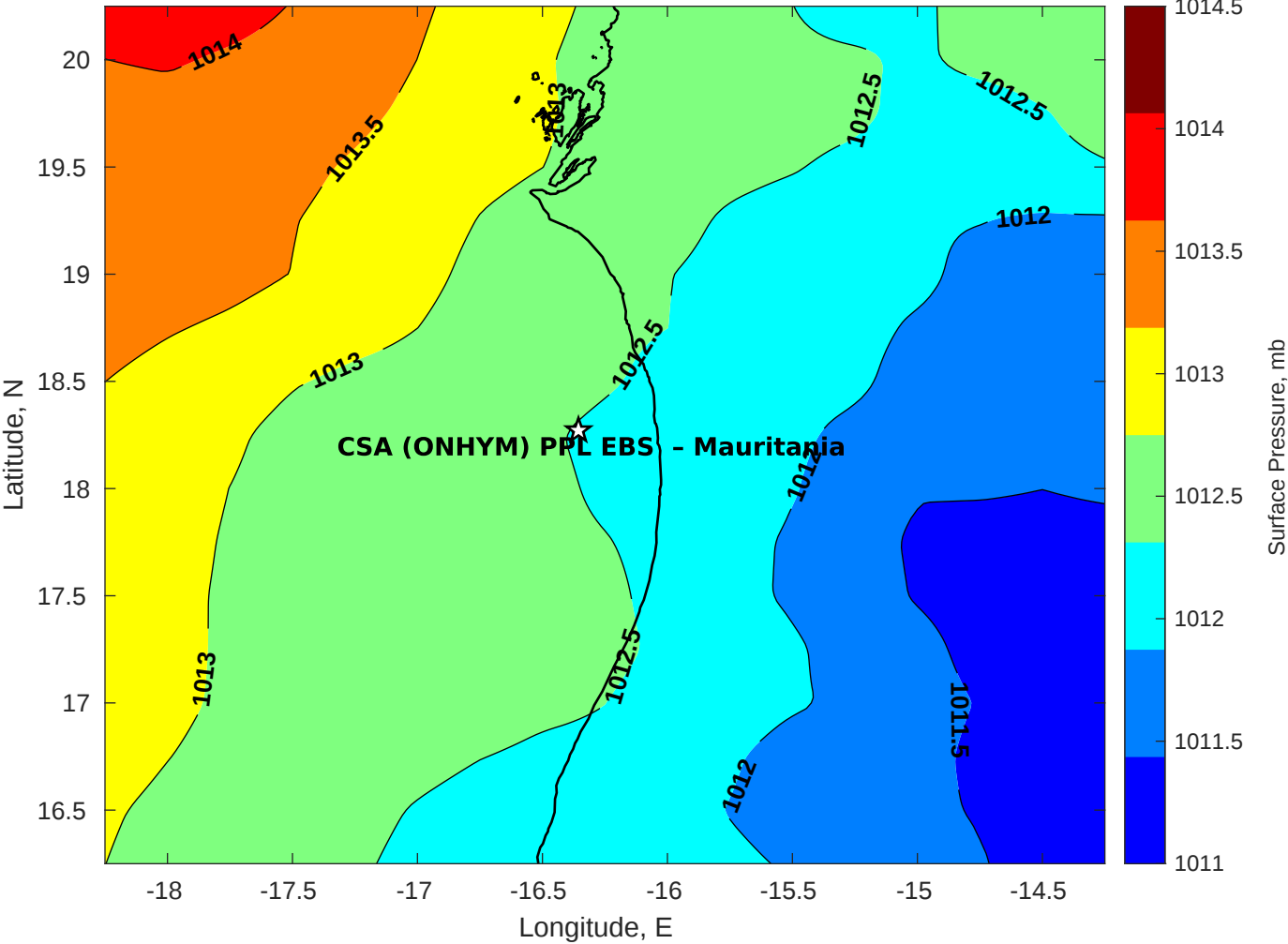
Surface Pressure (mb) for CSA (ONHYM) PPL EBS - Mauritania at 01-Nov-2025 00:00:00
