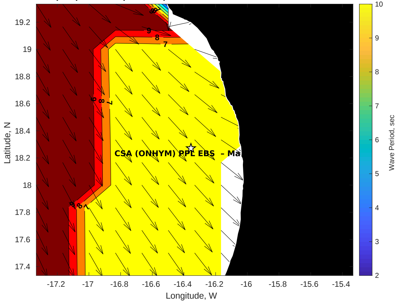
Wave Period (sec) for CSA (ONHYM) PPL EBS - Mauritania at 31-Oct-2025 09:00:00
