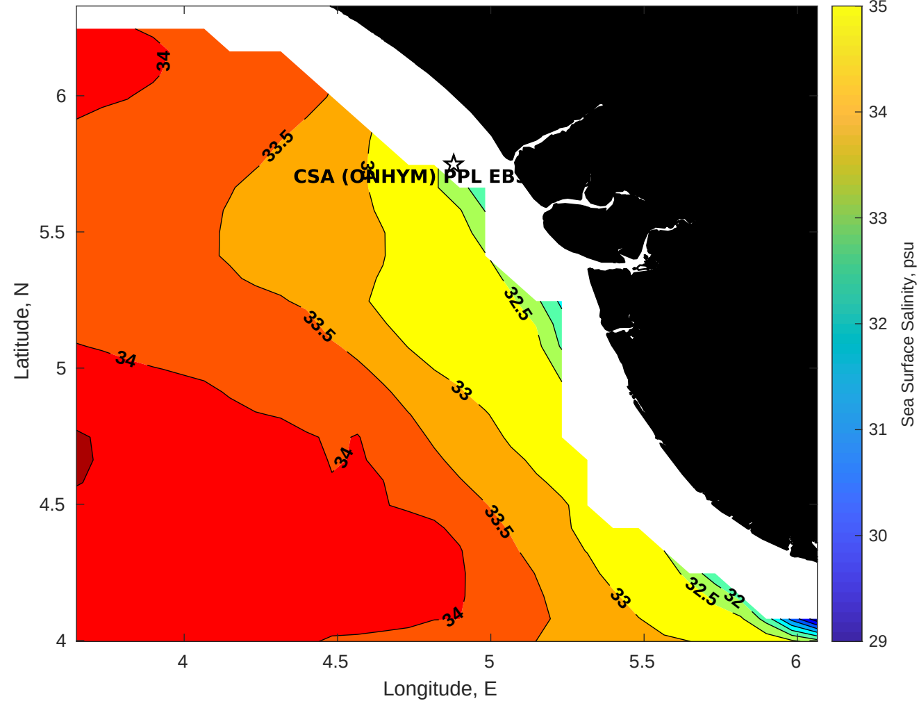
Surface Salinity for CSA (ONHYM) PPL EBS - Nigeria at 29-Oct-2025 00:00:00
