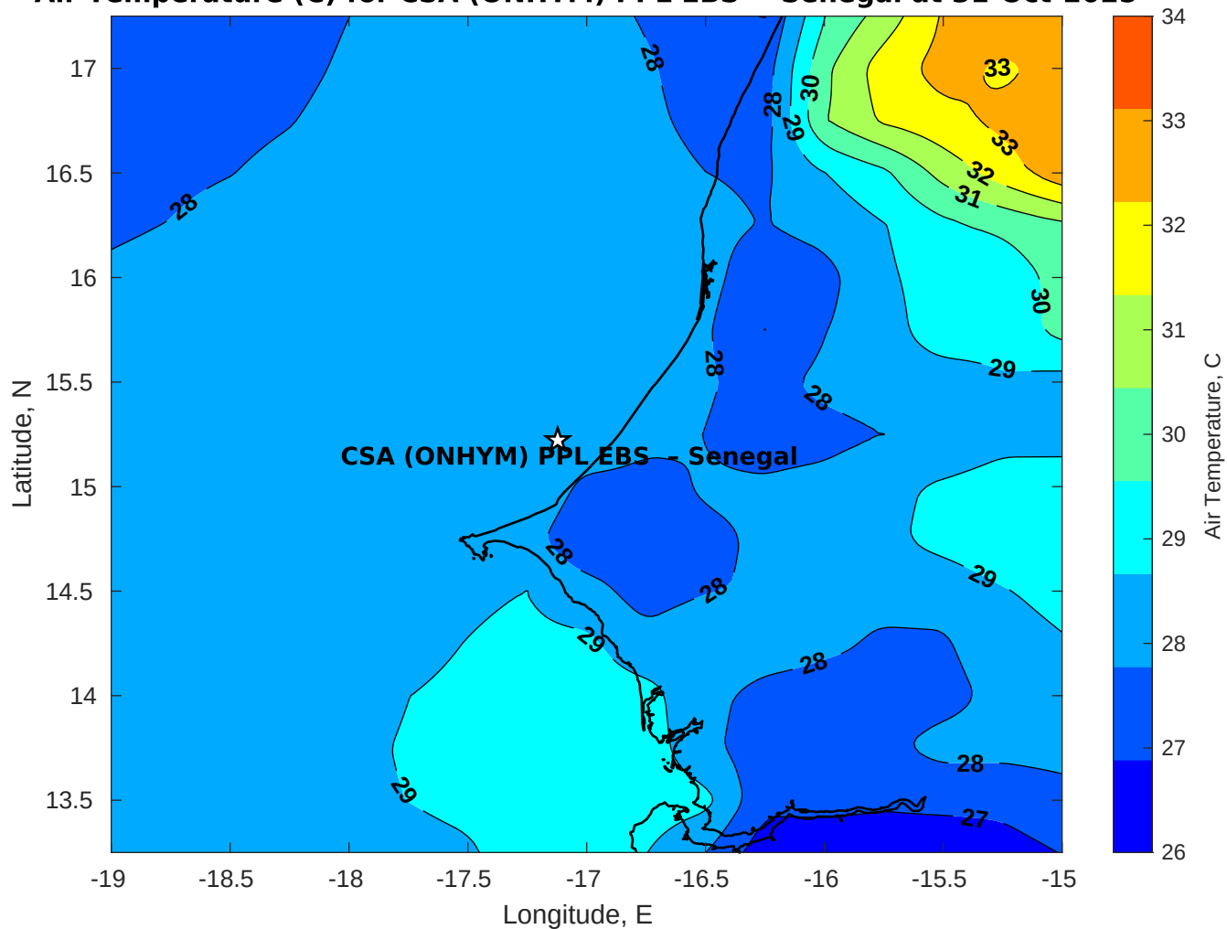
Air Temperature (C) for CSA (ONHYM) PPL EBS - Senegal at 31-Oct-2025
