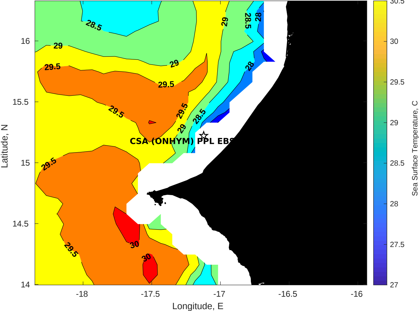
SST for CSA (ONHYM) PPL EBS - Senegal at 29-Oct-2025 00:00:00
