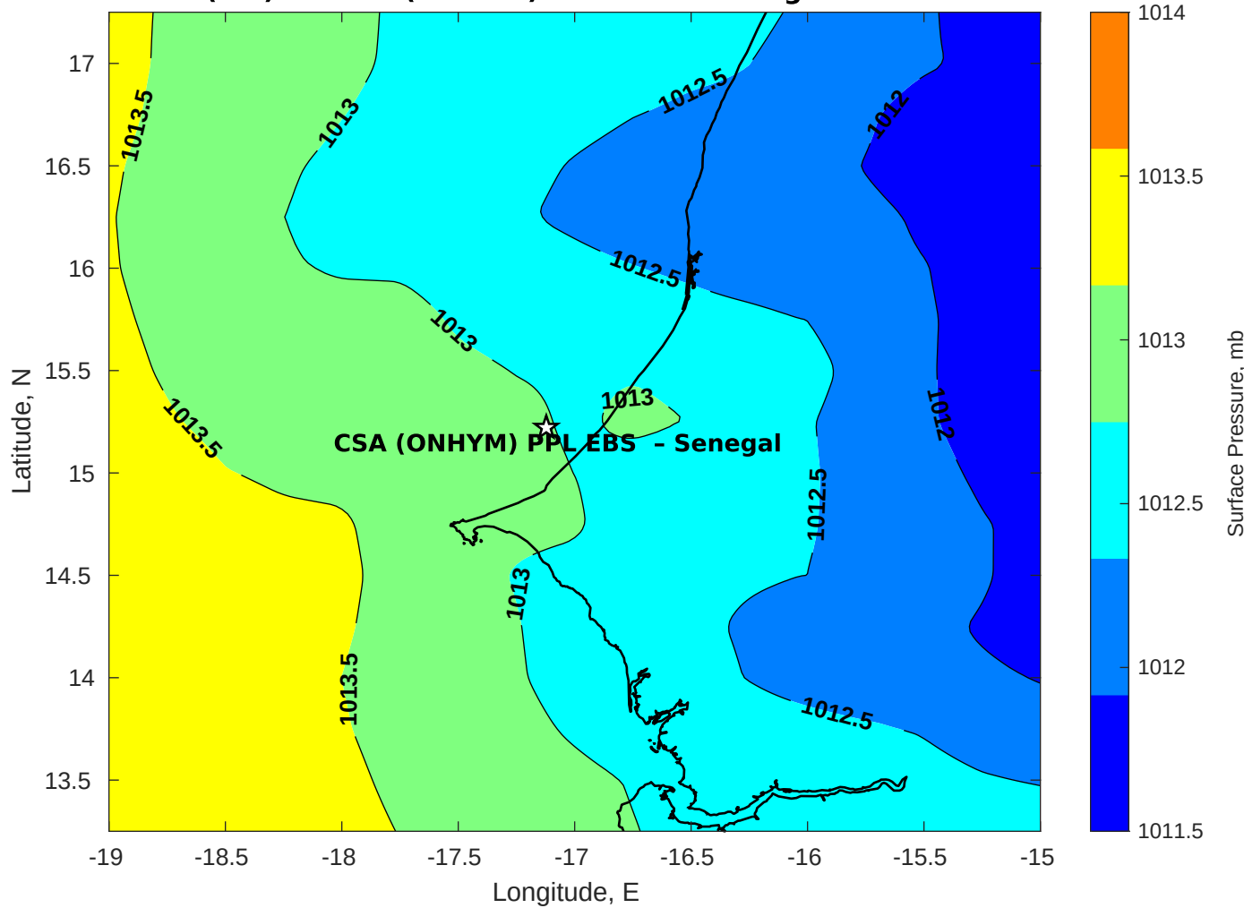
Surface Pressure (mb) for CSA (ONHYM) PPL EBS - Senegal at 01-Nov-2025 00:00:00
