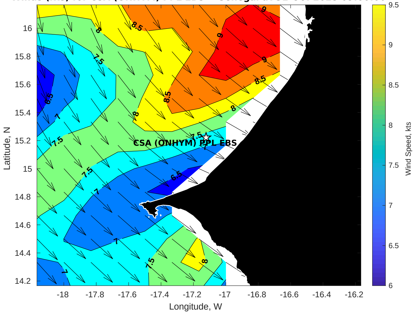
Winds (kts) for CSA (ONHYM) PPL EBS - Senegal at 31-Oct-2025 09:00:00
