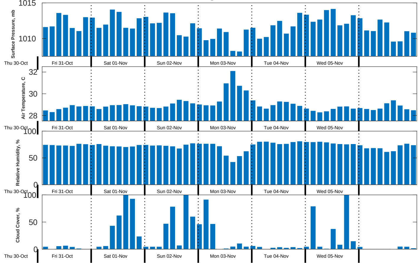
Met Forecast for CSA (ONHYM) PPL EBS - Senegal from 31-Oct-2025 00:00:00 to 07-Nov-2025 00:00:00
