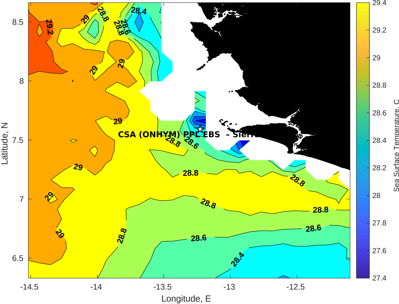
SST for CSA (ONHYM) PPL EBS - Sierra Leone at 29-Oct-2025 00:00:00
