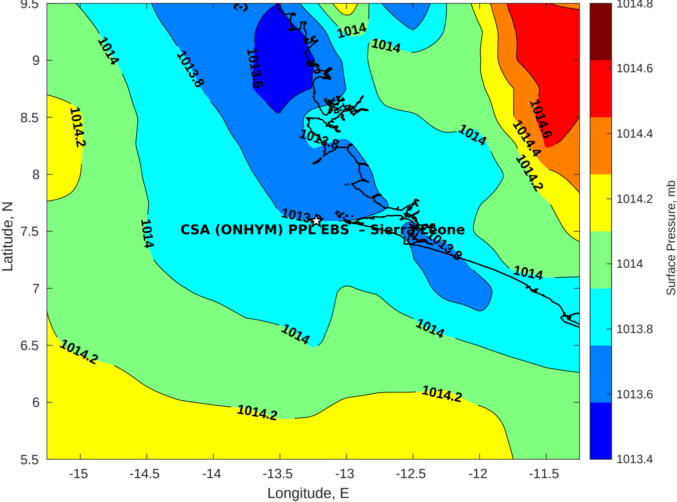
Surface Pressure (mb) for CSA (ONHYM) PPL EBS - Sierra Leone at 02-Nov-2025 00:00:00
