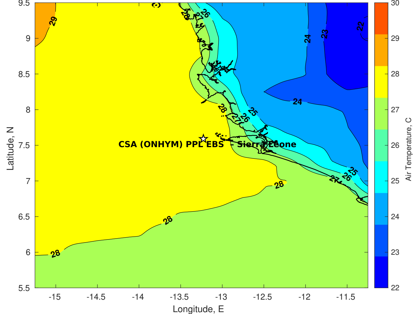
Air Temperature (C) for CSA (ONHYM) PPL EBS - Sierra Leone at 31-Oct-2025
