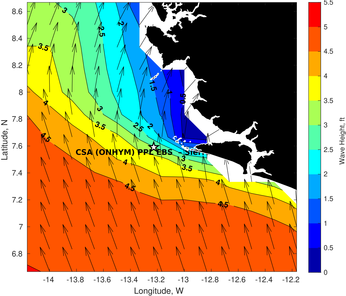
Wave Height (ft) for CSA (ONHYM) PPL EBS - Sierra Leone at 31-Oct-2025 09:00:00
