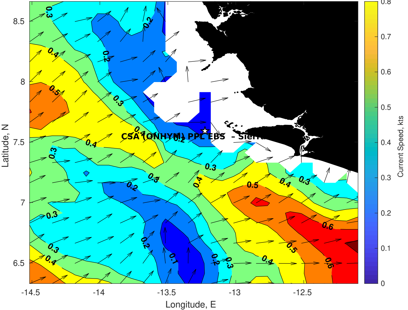
Surface Currents for CSA (ONHYM) PPL EBS - Sierra Leone at 29-Oct-2025 00:00:00
