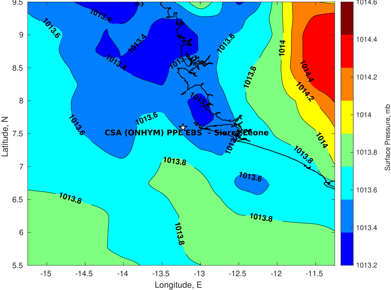
Surface Pressure (mb) for CSA (ONHYM) PPL EBS - Sierra Leone at 01-Nov-2025 00:00:00
