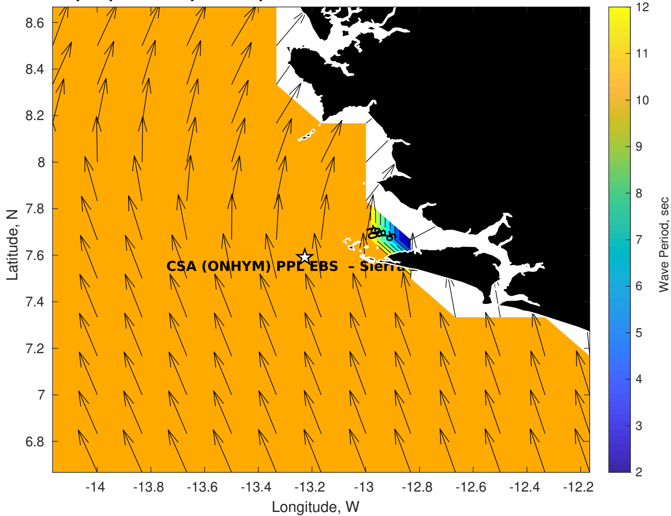
Wave Period (sec) for CSA (ONHYM) PPL EBS - Sierra Leone at 31-Oct-2025 09:00:00
