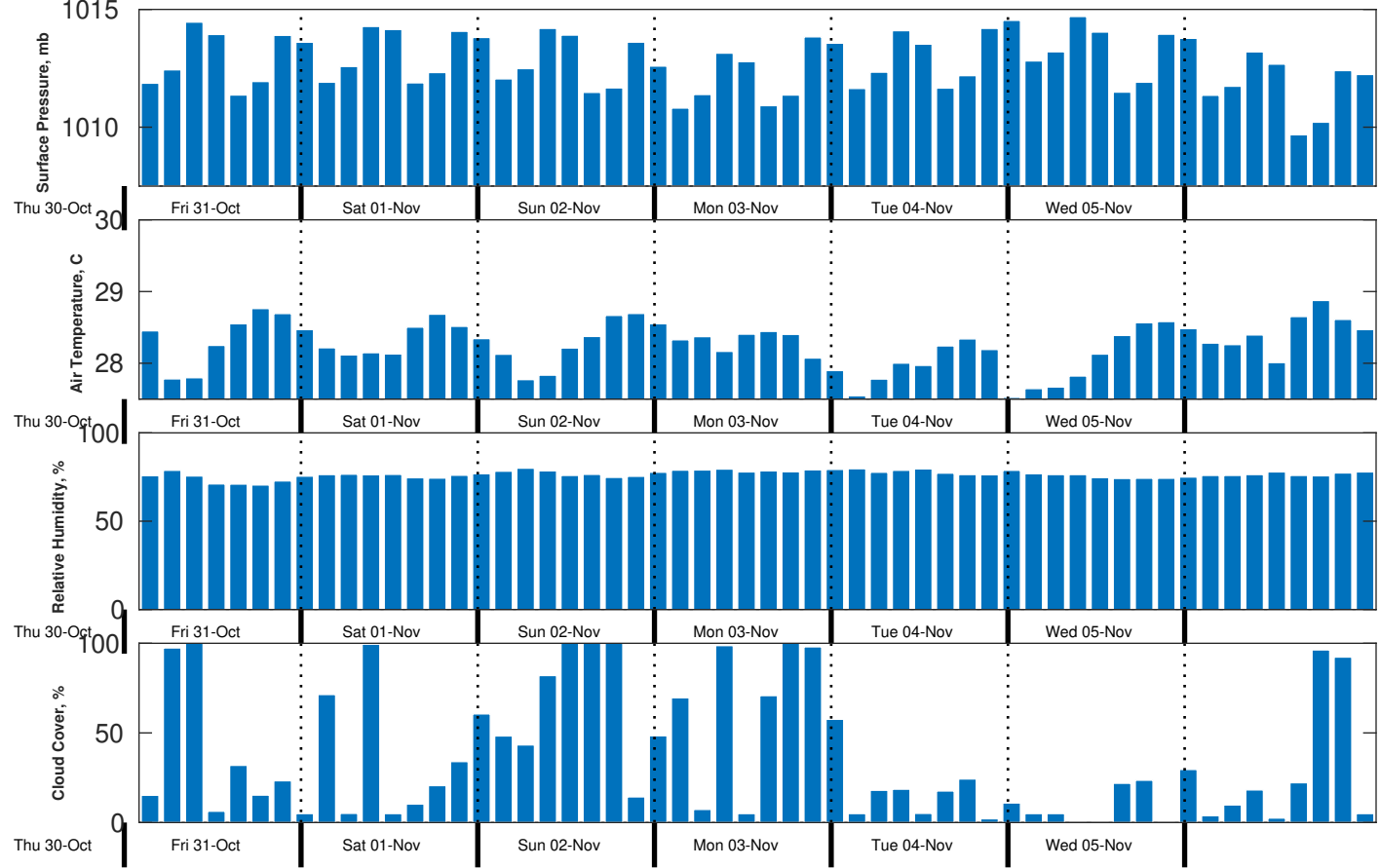
Met Forecast for CSA (ONHYM) PPL EBS - Sierra Leone from 31-Oct-2025 00:00:00 to 07-Nov-2025 00:00:00
