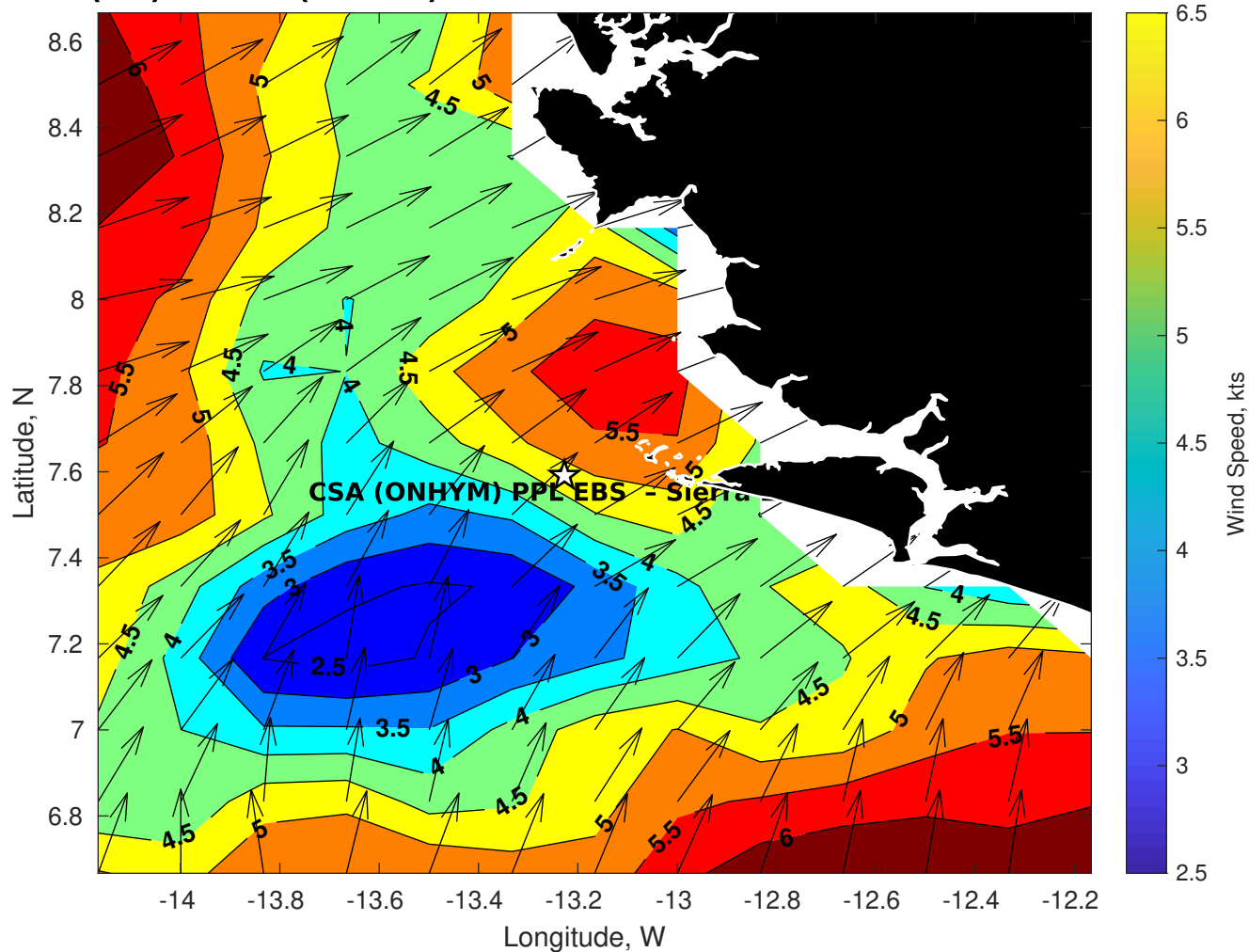
Winds (kts) for CSA (ONHYM) PPL EBS - Sierra Leone at 31-Oct-2025 09:00:00
