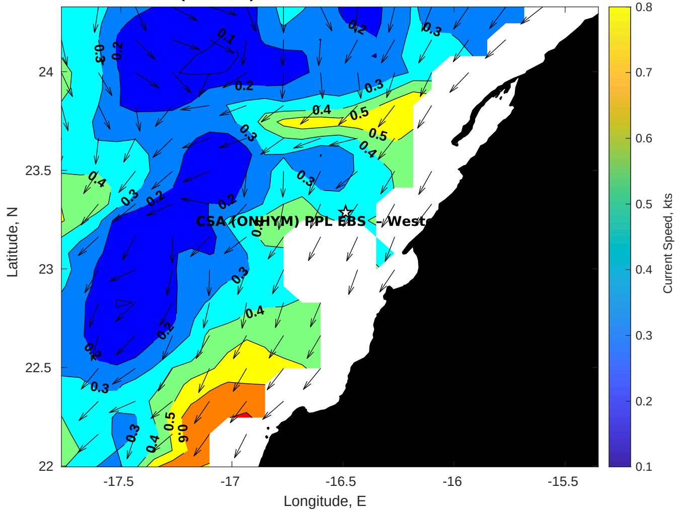
Surface Currents for CSA (ONHYM) PPL EBS - Western Sahara at 29-Oct-2025 00:00:00
