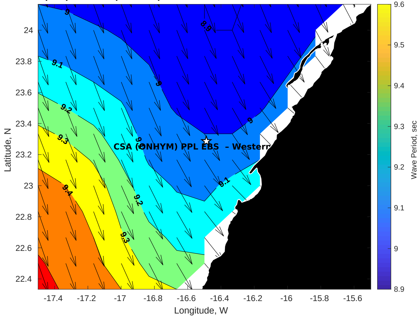
Wave Period (sec) for CSA (ONHYM) PPL EBS - Western Sahara at 31-Oct-2025 09:00:00
