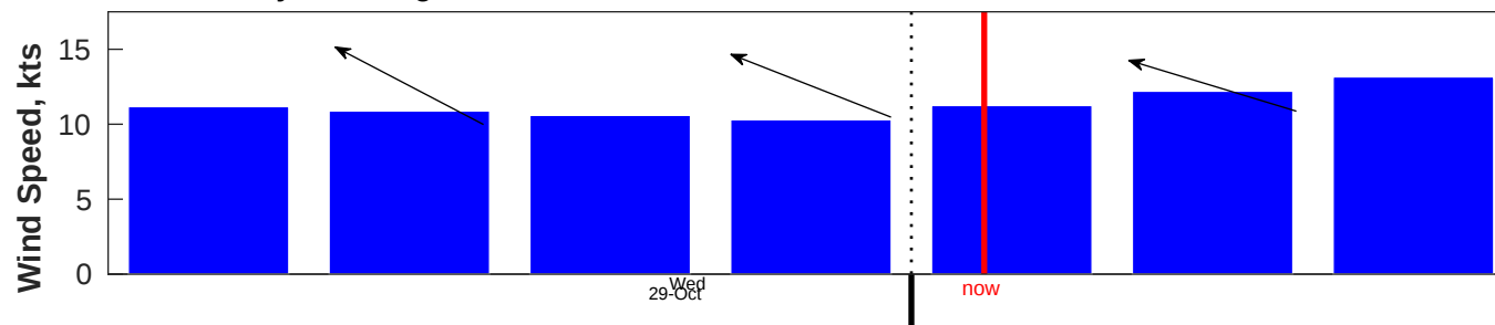
Wind & Wave Forecast for Gyre Passage: Dakar to Trinidad from 29-Oct-2025 19:00:00 to 30-Oct-2025 01:00:00
