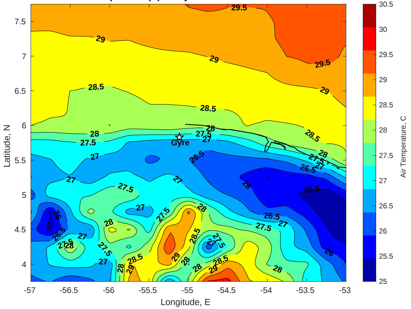
Air Temperature (C) for Gyre at 31-Oct-2025
