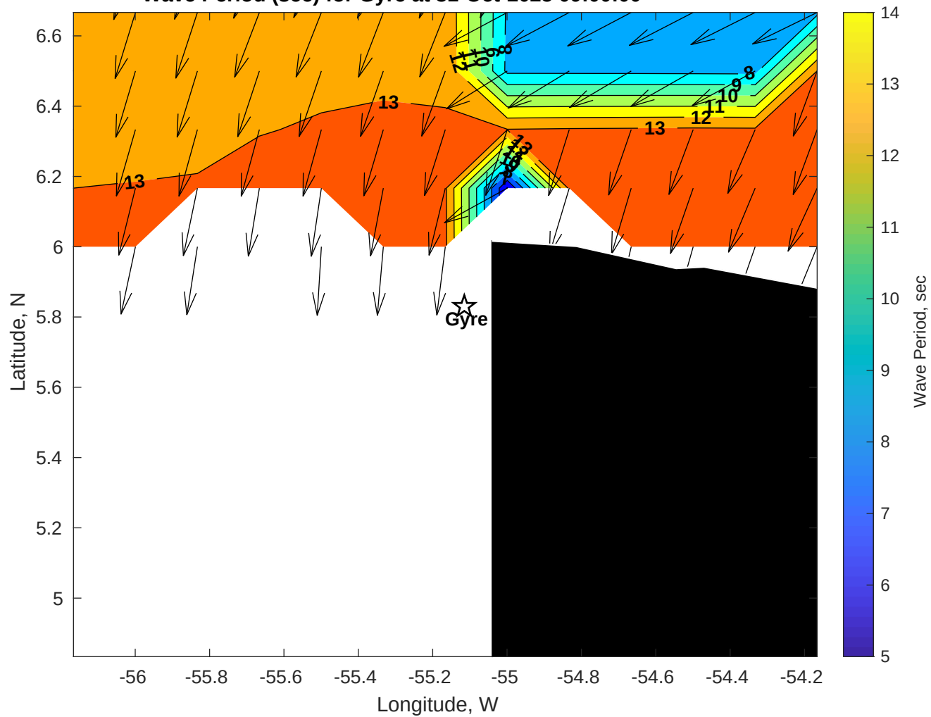
Wave Period (sec) for Gyre at 31-Oct-2025 09:00:00
