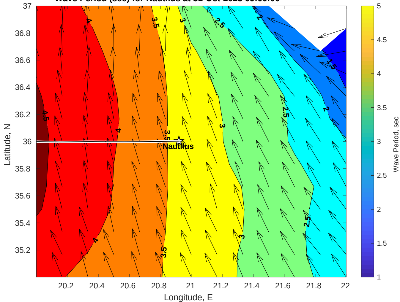
Wave Period (sec) for Nautilus at 31-Oct-2025 09:00:00
