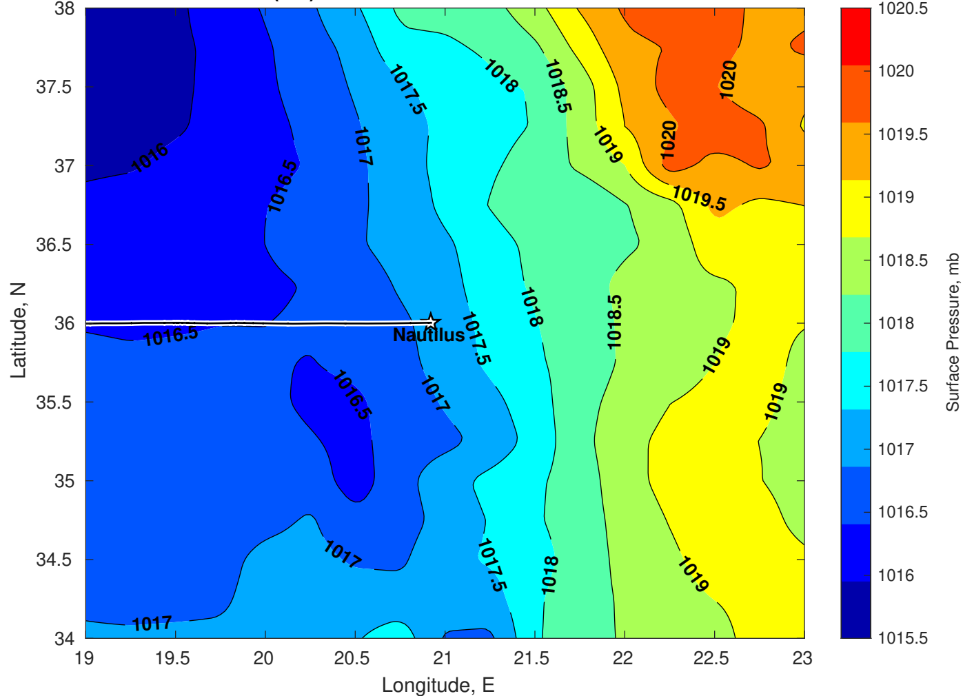
Surface Pressure (mb) for Nautilus at 01-Nov-2025 00:00:00
