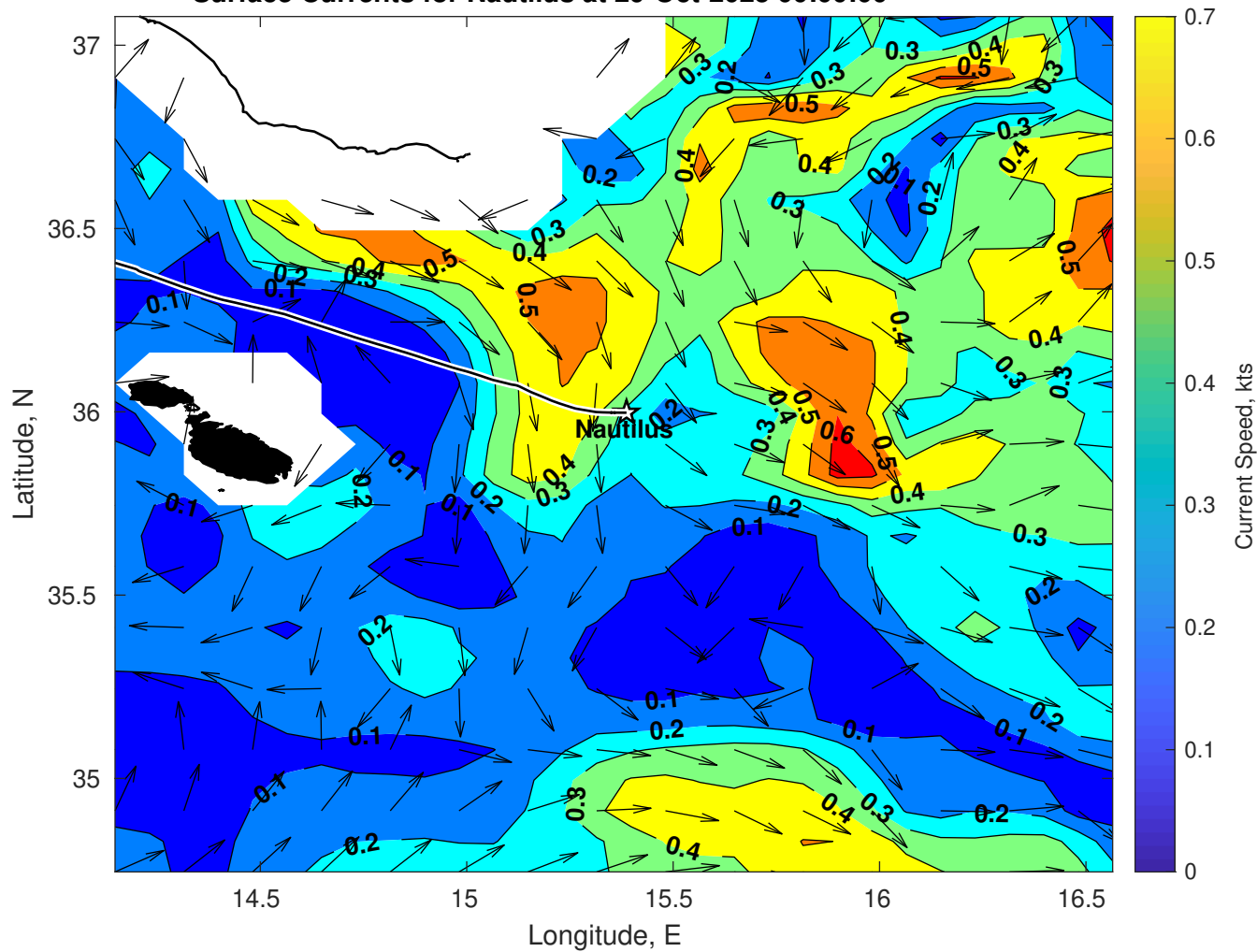
Surface Currents for Nautilus at 29-Oct-2025 00:00:00
