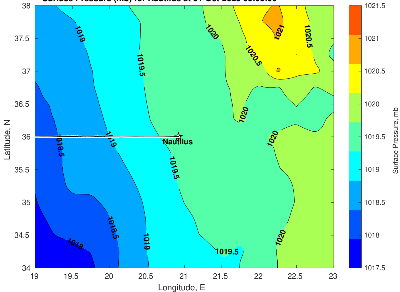
Surface Pressure (mb) for Nautilus at 31-Oct-2025 00:00:00
