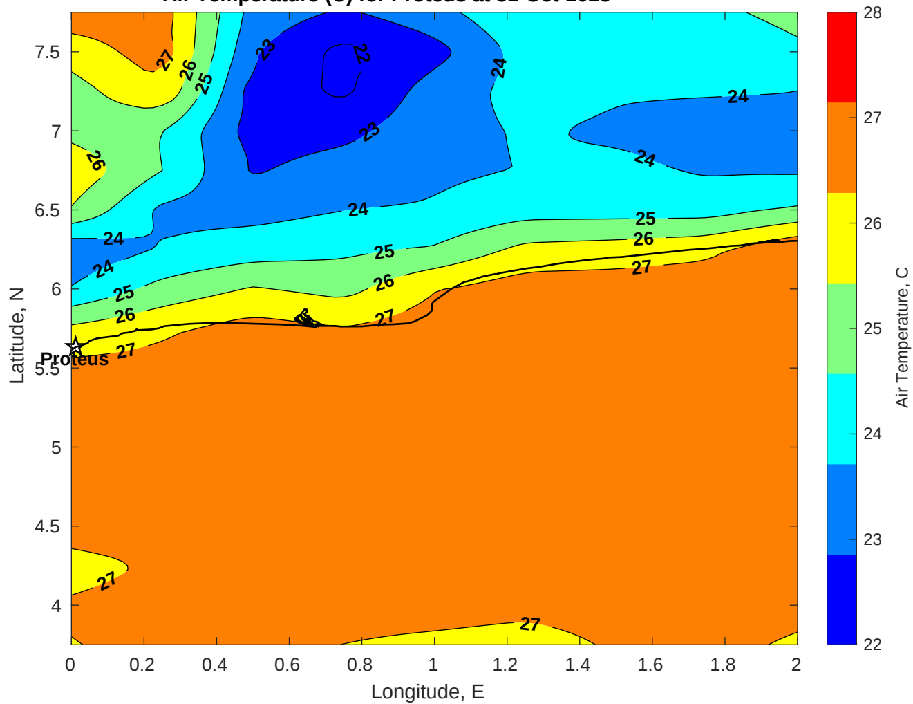
Air Temperature (C) for Proteus at 31-Oct-2025
