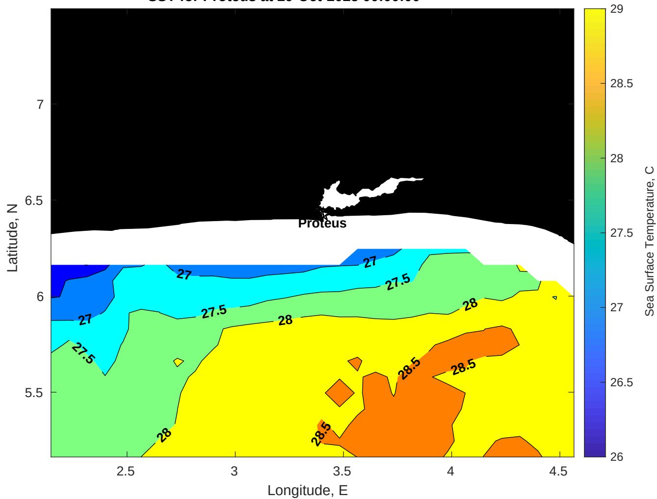
SST for Proteus at 29-Oct-2025 00:00:00
