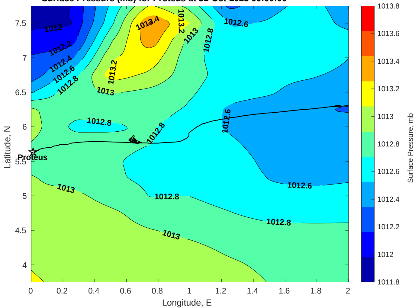
Surface Pressure (mb) for Proteus at 31-Oct-2025 00:00:00
