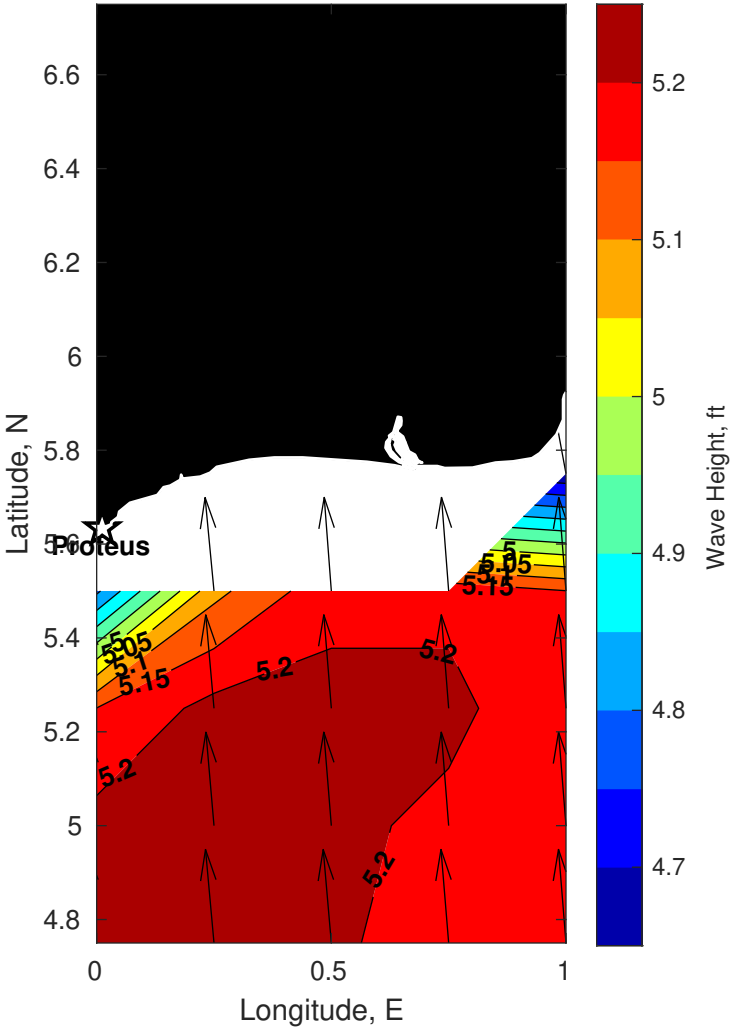
Wave Height (ft) for Proteus at 31-Oct-2025 09:00:00
