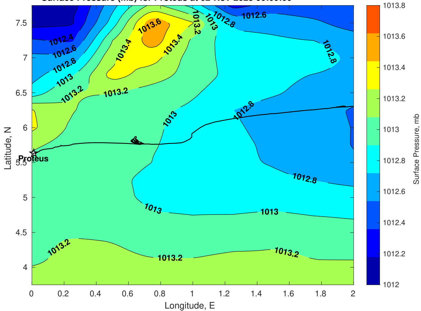
Surface Pressure (mb) for Proteus at 02-Nov-2025 00:00:00
