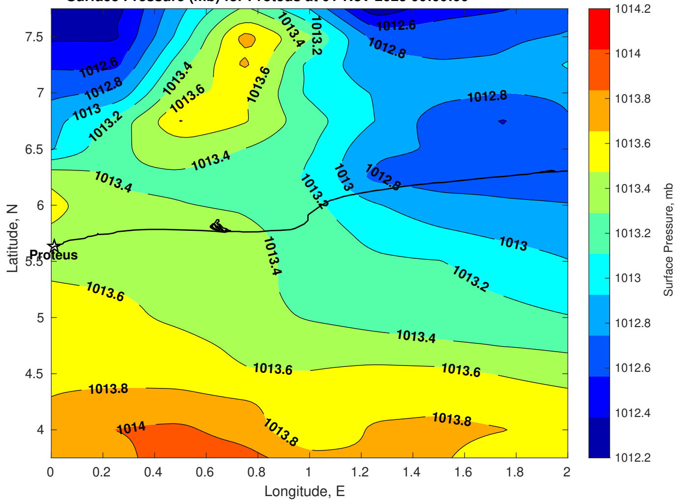
Surface Pressure (mb) for Proteus at 01-Nov-2025 00:00:00
