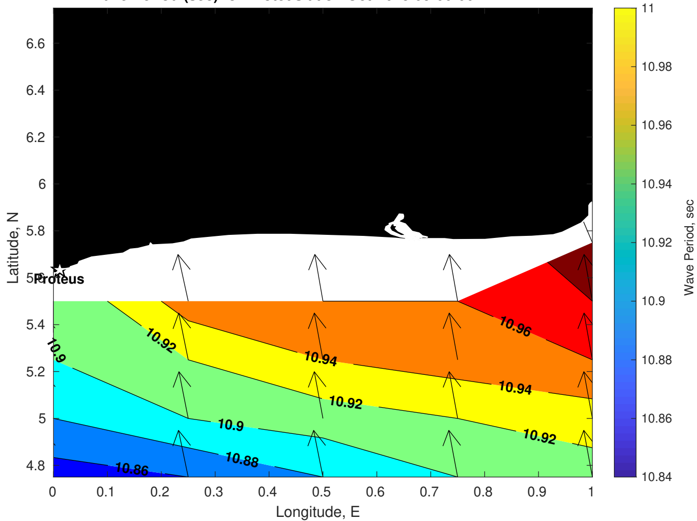
Wave Period (sec) for Proteus at 31-Oct-2025 09:00:00
