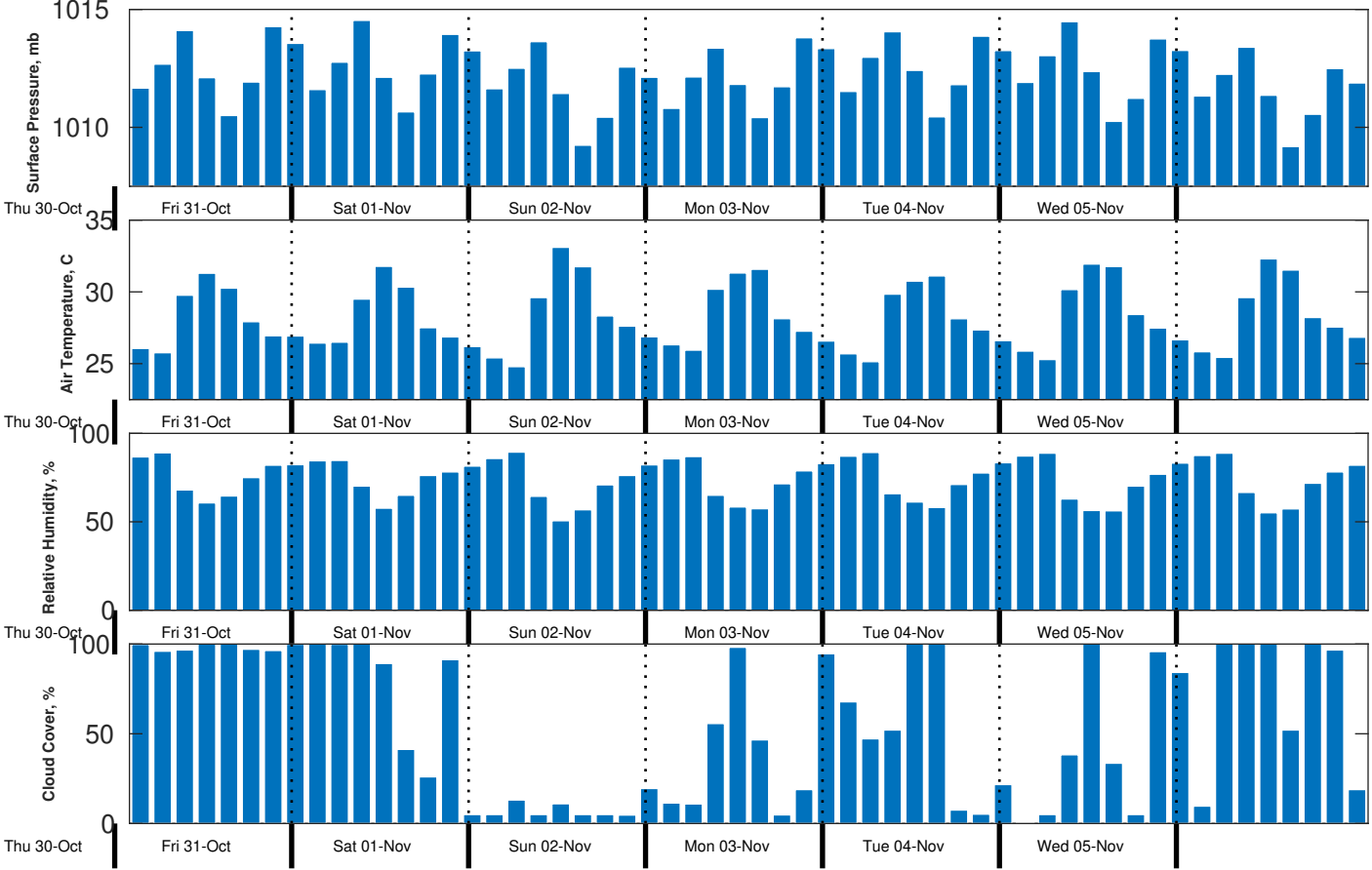
Met Forecast for Proteus from 31-Oct-2025 00:00:00 to 07-Nov-2025 00:00:00
