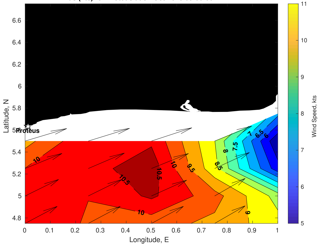
Winds (kts) for Proteus at 31-Oct-2025 09:00:00
