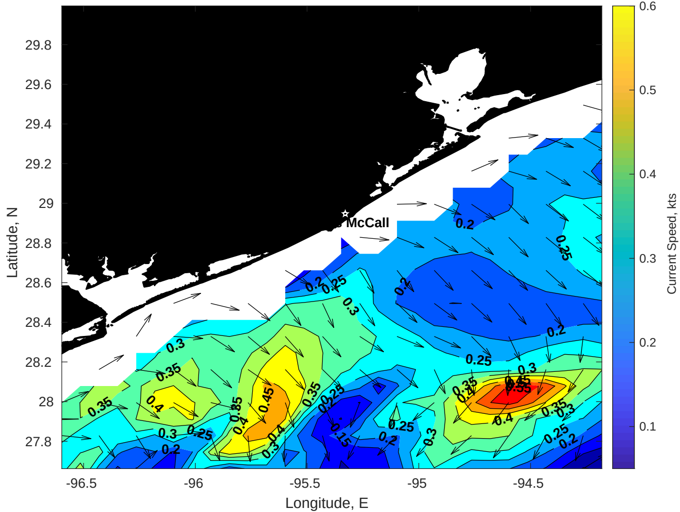
Surface Currents for Brooks McCall at 31-Oct-2025 00:00:00
