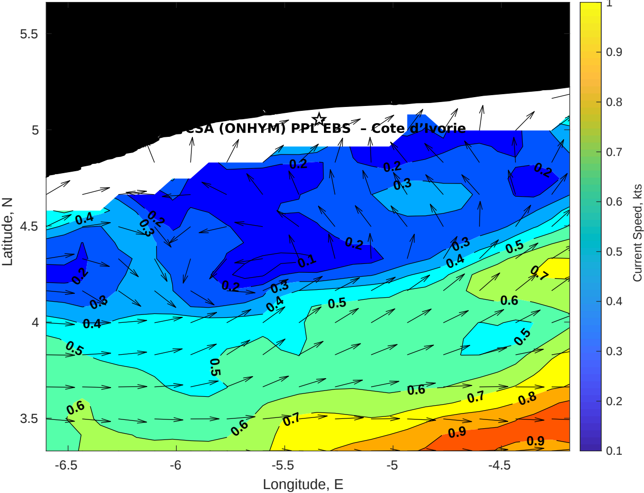
Surface Currents for CSA (ONHYM) PPL EBS - Cote d'Ivoire at 31-Oct-2025 00:00:00
